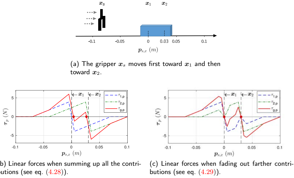
Figure 4.10: The figures show the linear haptic cues guiding the user toward grasping poses x_1 and x_2 as a function of the position of the gripper in a mono-directional case. They highlight the difference between a simple summation of the forces of attraction to all grasping poses (Fig. (b)) and the adopted solution, which centers the attraction force on the closest grasp candidate (Fig. (c)).
