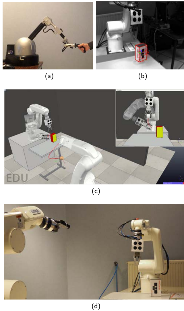
Figure 3.15: The figure shows the experimental setup used to validate the approach. (a) shows the master side whereas (b) shows the tracker used to retrieve the pose of the object to be grasped in real time. (c) shows the virtual environment reconstructed using the tracker's and kinematic data and used as an interface with the operator while (d) is the two slave manipulators arms along with the object to be grasped.
