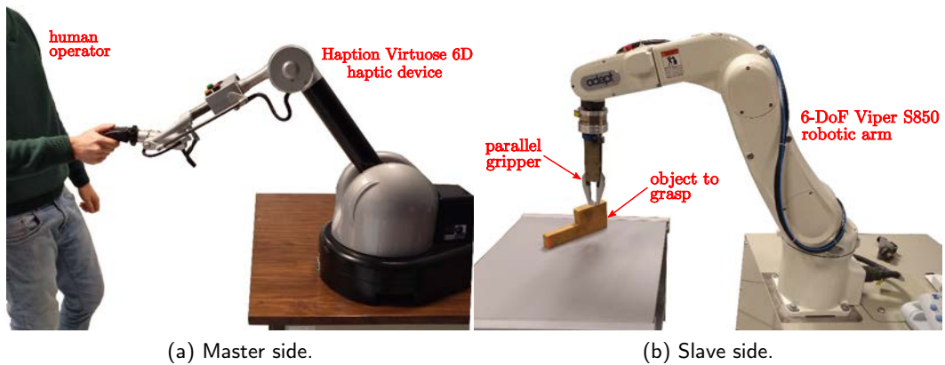
Figure 3.13: Experimental setup. The master system is composed of the Haption Virtuose 6D haptic device, while the the slave system is composed of a 6-DoF Viper S850 robotic arm carrying a pneumatic parallel gripper. A wooden object with dimensions 21 \times 9 \times 3 cm and weight 300 g is placed on a table in front of the robotic manipulator.
