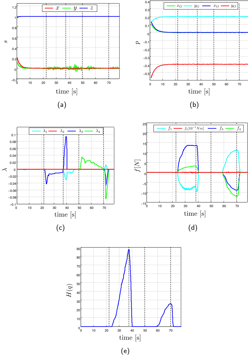
Figure 3.12: Results of the second experiment. (a) behavior of the primary task \mathbf{s}(t) ; (b) behavior of the gripper and object positions \mathbf{p} = [\mathbf{p}_g^T \ \mathbf{p}_o^T]^T on the image plane; (c) Behavior of the four operator's commands \boldsymbol{\lambda} for actuating the null-space directions \mathbf{n}_i . (d) Behavior of the four force cues f_i displayed to the human operator during the robot motion; (e) behavior of the scalar cost function H(\mathbf{q}) quantifying the proximity to joints limits.
