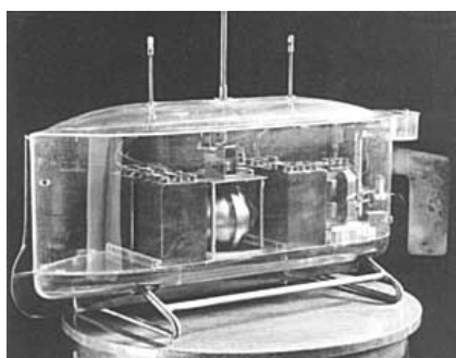
Figure 1.3: Tesla's Boat. Photo courtesy [13].
