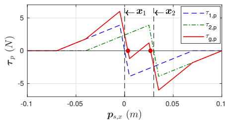
(b) Linear forces when summing up all the contributions (see eq. (4.28)).
