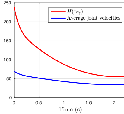
Figure 5.4: Behaviour of the cost function H(o \mathbf{x}_g) and of the average joint velocity: note how H(o \mathbf{x}_g) monotonically decreases as the user follows the provided force cues (as expected). Consequently, also the integral joint velocity norm decreases as well, as the gripper reaches an optimal pose.
