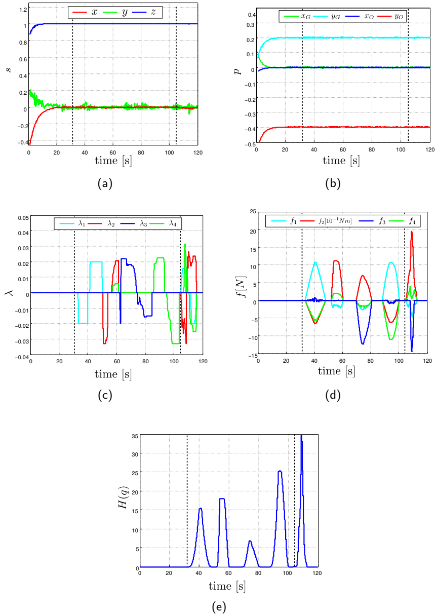
Figure 3.11: Results of the first experiment. (a) behavior of the primary task s(t) ; (b) behavior of the gripper and object positions \bar{p} = [\bar{p}_g^T \bar{p}_o^T]^T on the image plane; (c) Behavior of the four operator's commands \lambda for actuating the null-space directions n_i . (d) Behavior of the four force cues f_i displayed to the human operator during the robot motion; (e) behavior of the scalar cost function H(q_g, q_c) quantifying the proximity to joints limits.
