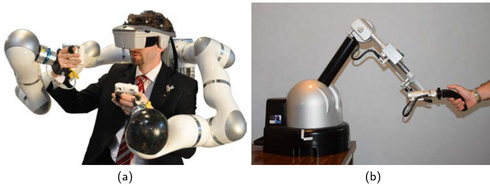
Figure 2.2: Examples of kinesthetic haptic devices. (a) HUG, a dual-arm kinesthetic haptic device built by DLR. Photo courtesy [52]. (b) Virtuuous 6D, a 6-DoF haptic device by haption [53].
