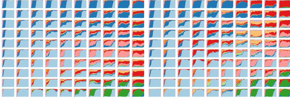
Figure 4.13: PCA relational SOM performed through a Nyström approximation using 1% (left) and 5% (right) of the observations: For each neuron of the map, job trajectories distribution is represented using the observations classified in the corresponding unit. Colors represent the type of contract.
