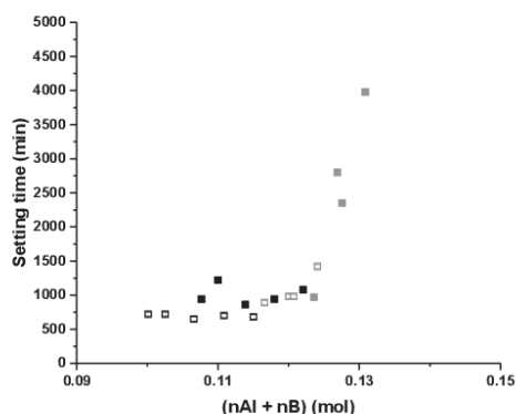
Figure 4. Evolution of setting time according to the aluminum and boron molar amount for (□) GM1 0.5 A650 0.5 and (■) GM1 0.7 A650 0.3 samples in presence of (■) one additive or (■) two additives (error +/- 30 min).
