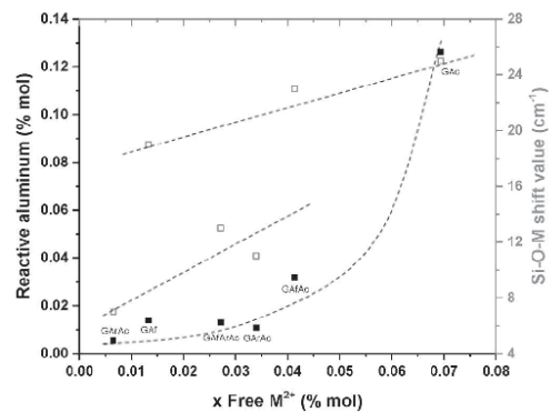
Fig. 9: (■) Rate of reactive aluminum and (□) FTIR shift of the Si-O-M bonds according to the molar percent of free \text{M}^{2+} cations (Ca or Mg) in the different samples GAr, \text{GAR}_{0.5}\text{Ac}_{0.5} , \text{GAR}_{0.5}\text{Ac}_{0.5} , GAc, \text{GAR}_{0.5}\text{Ar}_{0.33}\text{Ac}_{0.33} and \text{GAR}_{0.5}\text{Ar}_{0.33}\text{Ac}_{0.33} samples after seven days.
