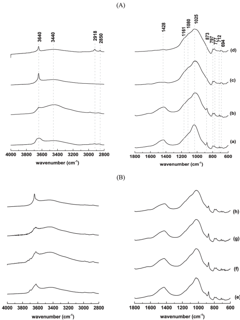
Fig. 4. FTIR spectra of (A) (a) 600A, (b) 700A (c) 750A and (d) 800A furnace heated argillite samples and (B) (e) F600A, (f) F650A (g) F700A and (h) F750A flash heated samples.
