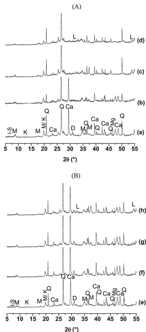
Fig. 5. XRD patterns of (A) (a) ^{600}\text{A} , (b) ^{700}\text{A} , (c) ^{750}\text{A} and (d) ^{800}\text{A} furnace heated argillite samples and (B) (e) ^{750}\text{A} , (f) ^{750}\text{A} , (g) ^{750}\text{A} and (h) ^{750}\text{A} flash heated samples. JCPDS files (Q: Quartz (04-016-2085), I-S: Illite-Smectite, K: Kaolinite (00-012-0447), M: Muscovite (00-003-0849), Ca: Calcite (00-005-0586), Mg: Magnesite (04-012-4921), L: Lime (01-082-1690), D: Dolomite (04-015-9852)).
