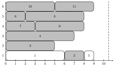
Figure 2.4: Optimal solution for JACKSON, |\hat{V}^1| = 6 and |\hat{W}| = 3 .
