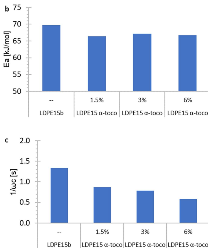
Figure 4.60. Rheological properties of LDPE 15 with and without (w/o) \alpha -tocopherol in formulation. a. zero shear viscosity ( \eta_0 ) b. energy of activation (Ea) c. relaxation time ( 1/\omega_c ). *LDPE 15 b extruded w/o antioxidant).
