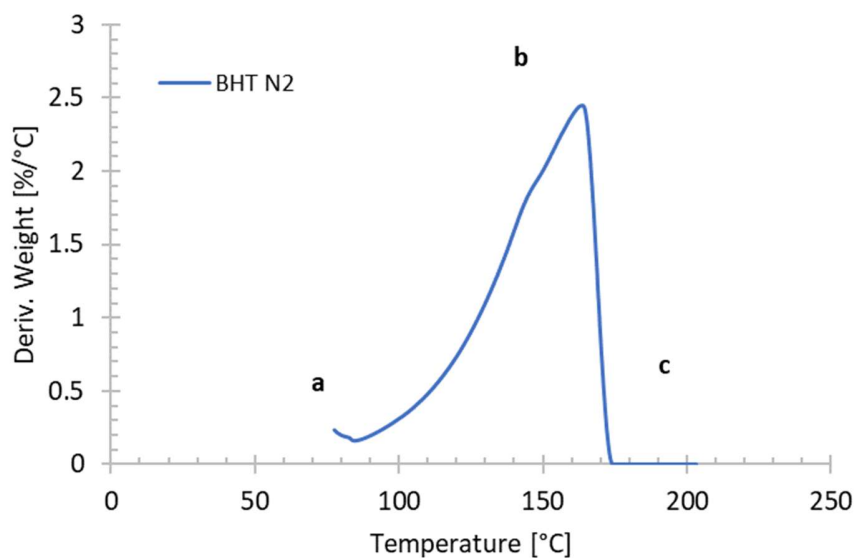
Figure 4.30. dTGA thermograms of the thermal degradation of BHT in nitrogen (N 2 ). a. Tonset, b. Tmax, c. Tendset.
