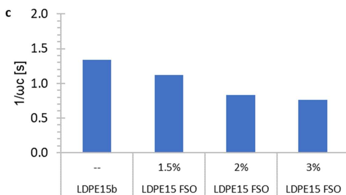
Figure 4.59. Rheological properties of LDPE 15 with and without (w/o) FSO in formulation. a. zero shear viscosity ( \eta_0 ) b. energy of activation ( E_a ) c. relaxation time ( 1/\omega c ). *LDPE 15 b extruded w/o antioxidant).
