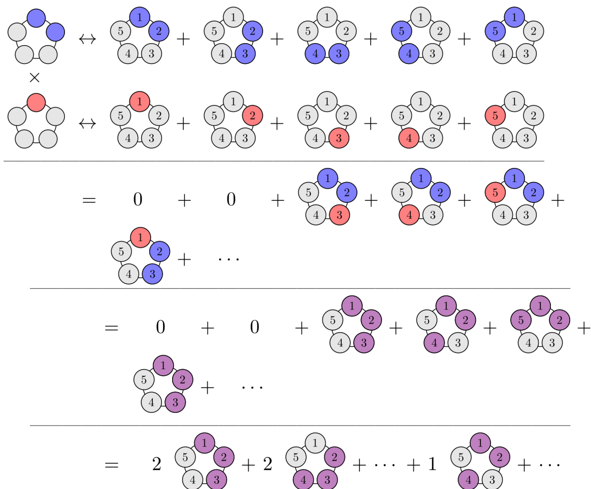
Figure 3.4: Example of an orbital product on the finite case of C_5
