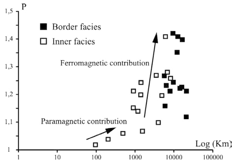
Figure III-16: P(K_m) diagram showing a broad correlation between P (degree of anisotropy) and K_m values due to the iron content of ferromagnetic minerals and paramagnetic mafic silicates.
