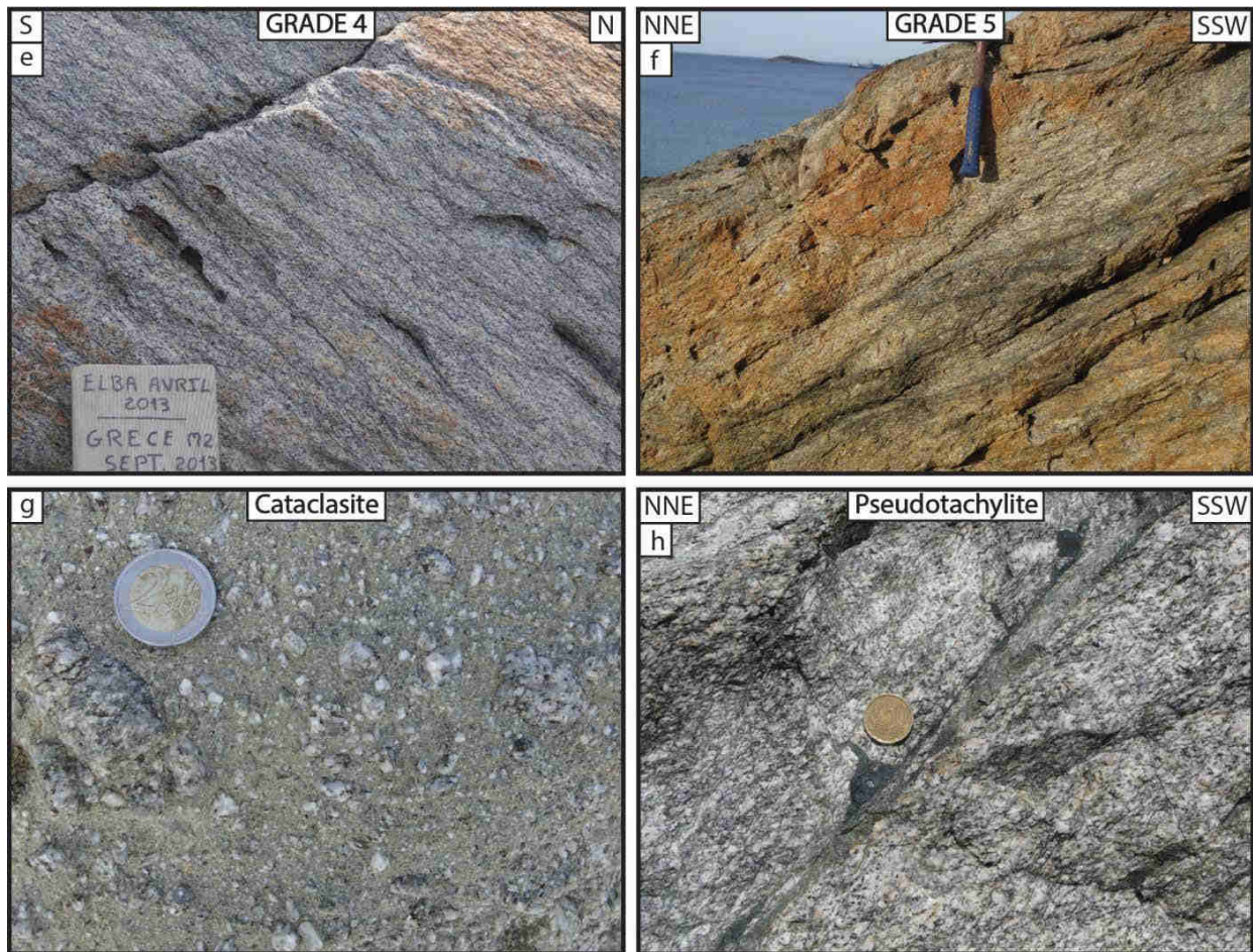
Figure II-5: presentation of the deformation intensity scale with field pictures. (a) Grade 0: isotropic magmatic fabric. (b) Grade 1: anisotropic magmatic deformation. (c) Grade 2: first strain localization with ductile deformation. (d) Grade 3: first shear bands. (e) Grade 4: first ultramylonitic bands. (f) Grade 5: intensification and development of ultramylonitic bands. (g) Cataclasite. (h) Pseudotachylite veins.
