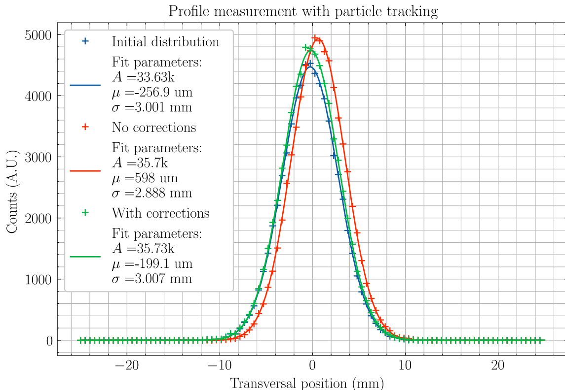
Figure 3.17 – Particle tracking for real symmetric field configuration with and without correctors (degraders and disks). The proton beam is assumed to be gaussian with \sigma_{beam} = 3 \text{ mm} . When no correction are applied, the mean value and the \sigma_{beam} are less affected compare to the asymmetric case. When correctors are present, the mean value is kept ( < 50 \mu\text{m} ) and the error on the \sigma_{beam} is less than 20 \mu\text{m} .
