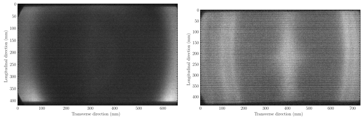
(a) Profile measurement attempt with electrons, Hamamatsu MCP.
