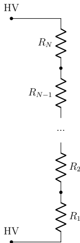
Figure 3.15 – Resistor chain.
