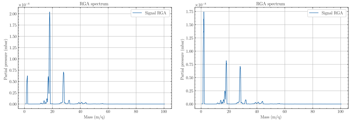
(a) An RGA spectrum dominated by water (high peaks at 18 17). Hydrogen (peak at 2) and nitrogen (peak at 28) are also present, as well as some heavy carbonate species (peaks above > 28 ).
