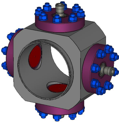
Figure 2.11 – A 3d drawing of the ESS button BPMs designed at DESY.
