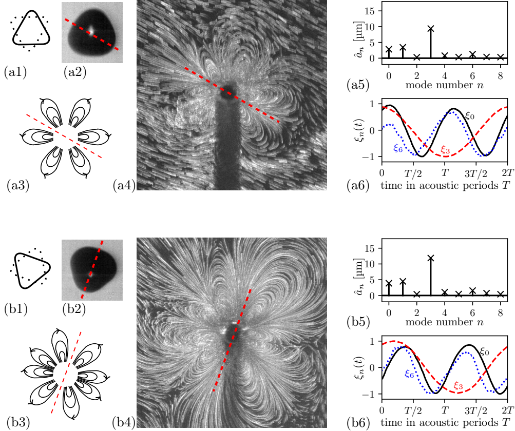
Figure 3.9: Presentation of four different streaming patterns observed for a bubble oscillating in a mode 3: case (a) – pattern with six lobes confined around the bubble ( R_0 = 70.8 \mu\text{m} , p_a = 9.2 \text{ kPa} ); case (b) – pattern with eight lobes confined around the bubble ( R_0 = 70.1 \mu\text{m} , p_a = 12.4 \text{ kPa} ); case (c) – cross-shaped pattern without any lobes ( R_0 = 65.7 \mu\text{m} , p_a = 15.1 \text{ kPa} ); case (d) – cross-shaped pattern with four circular zones of recirculation ( R_0 = 68.6 \mu\text{m} , p_a = 13.3 \text{ kPa} ). For each case (x), the information is structured as follows. (x1) schematic drawing of the bubble dynamics, and (x2) representative snapshot of the dynamics (image size 180 \mu\text{m} \times 180 \mu\text{m} ); (x3) schematic drawing of the streaming patterns, and (x4) streak photography of the streaming pattern (image size 1 \text{ mm} \times 1 \text{ mm} , 723 images corresponding to 1.2 ms of signal); (x5) maximum modal amplitudes; (x6) temporal evolution of: black line – \xi_0 , red dashed line – \xi_3 , and blue dotted line – \xi_6 .
