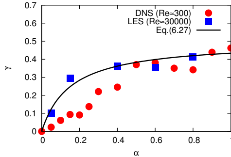
FIGURE 6.11: Energy ratio \gamma = E_T/E_P plotted as a function of \alpha at c_T = 0 and c_P = 0.04 : comparison between DNS ( \text{Re} \approx 300 ), LES ( \text{Re} \approx 30000 ) and Eq.(6.27) (with \lambda = 0.5 and d_T/c_\Pi = 0.15 ).
