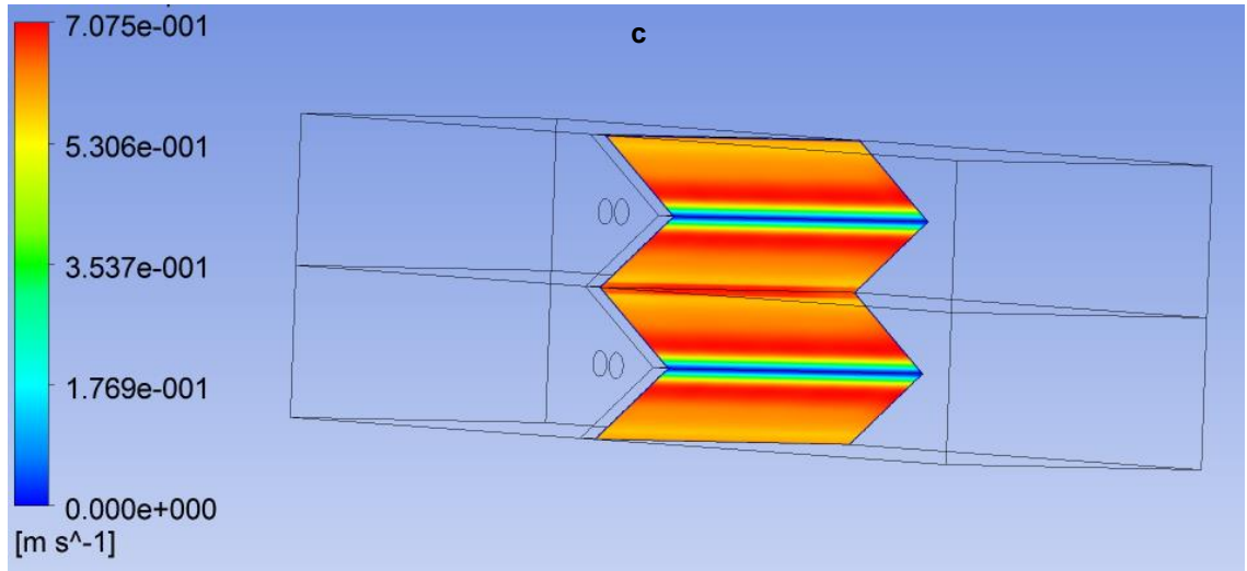
Figure 72 : Velocity contour showing flow behavior on the outlet of the media for the pleated configuration
