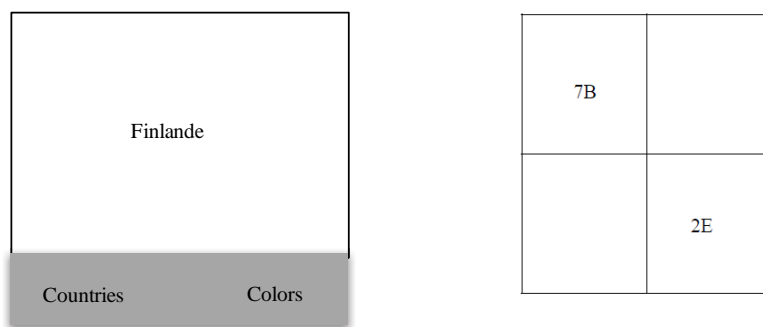
Figure 1: Representation of the Antisaccade task ( Top ), the Keep-track task ( Bottom left ) and Number-Letter task ( Bottom right ).
