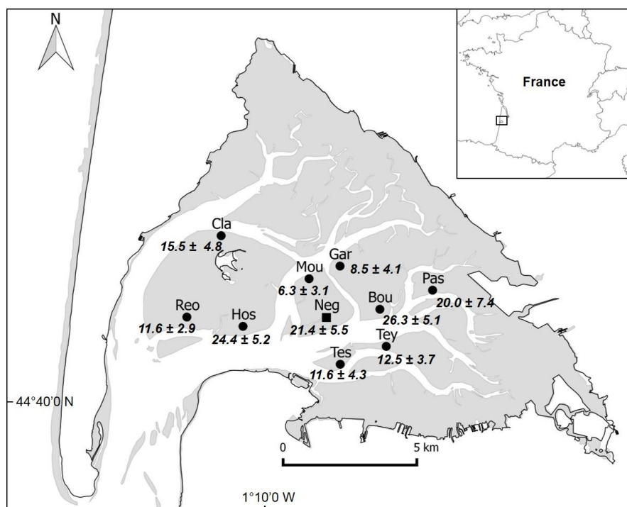
Figure III-A. 1 Location of study sites in Arcachon Bay, France. Square indicates location of temporal survey site (January 2014–December 2015). Prevalence (% ± SE) of bopyrid infestation in Upogebia cf. pusilla given for each station: Bou: Bourrut; Cla: Le Cla; Gar: Garrèche; Hos: Les Hosses; Mou: Les Moussettes; Neg: La Nègue; Pas: Passant; Reo: La Réousse; Tes: Le Tes; Tey: Le Teychan. Light grey: intertidal area. N = 30 –121 depending on study site.
