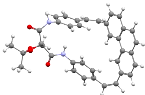
340b [AM1, RHF] \Delta H_f = +9,13 kcal/mol
