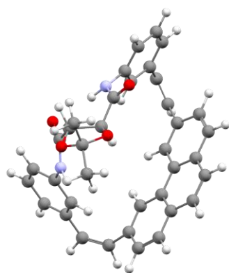
340a [AM1, RHF] \Delta H_f = +7,14 kcal/mol
