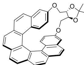
(S,S,M)-(-)- 353M
