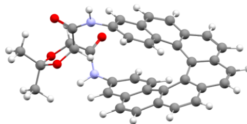
341a [AM1, RHF] \Delta H_f = +27,29 kcal/mol \varphi_{1-5} = +14^\circ; +18^\circ; +28^\circ; +23^\circ; +15^\circ
