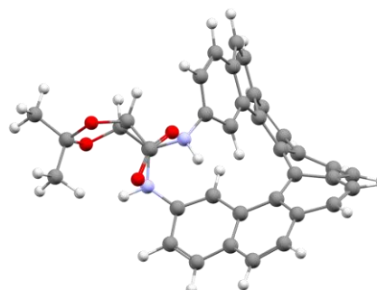
341b [AM1, RHF] \Delta H_f = +59,84 kcal/mol \varphi_{1-5} = -26^\circ; +21^\circ; +65^\circ; -5^\circ; -33^\circ
