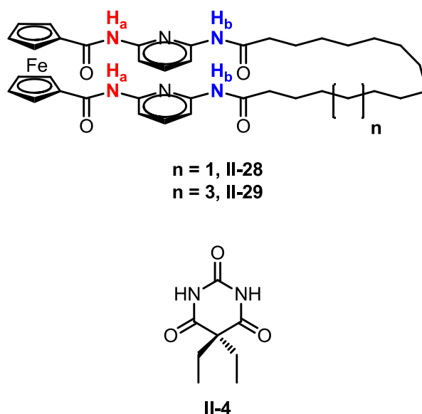
Figure 2.14 - Structural formulae of macrocyclic receptors II-28 and II-29 and barbitol. \text{H}_a and \text{H}_b denote protons used to follow guest binding in NMR studies.
