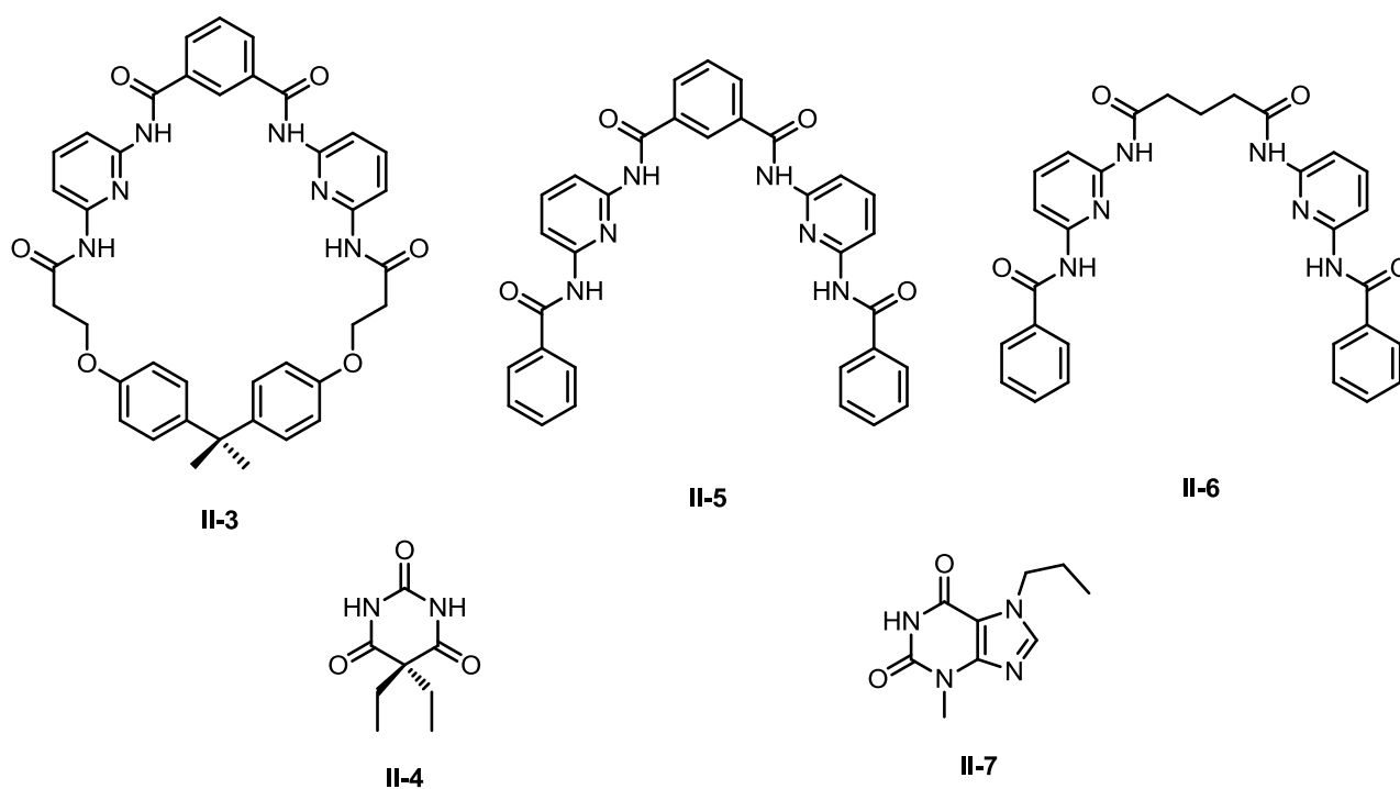
Figure 2.3 - Hamilton-type receptors II-3 , II-5 and II-6 , barbitol II-4 and 3-methyl-7-propylxanthine II-7 .
