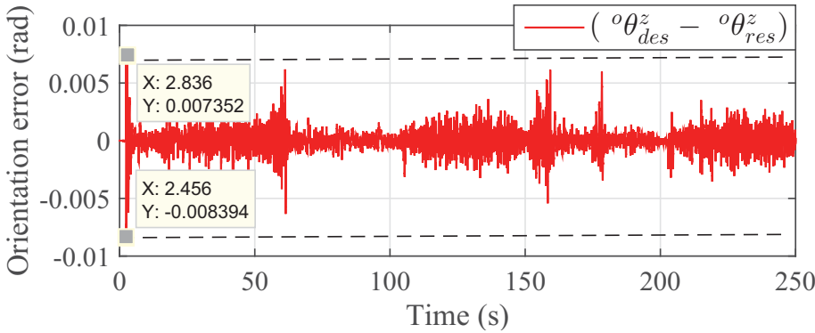
(b) Orientation tracking error
