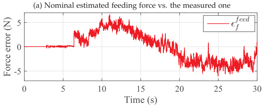
Figure 3.47: Feeding force variation
