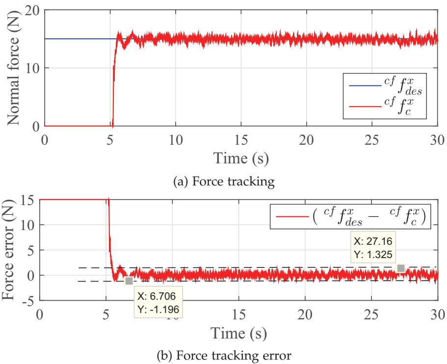
Figure 3.44: Force control performance in tracking the desired force value
