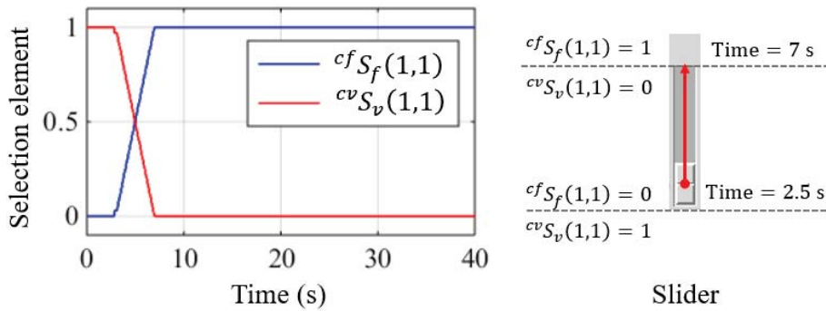
Figure 3.43: Switching from velocity to force control using interactive slider
