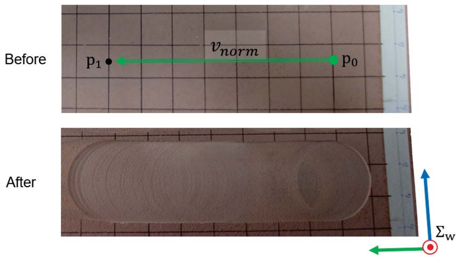
Figure 3.48: Flat wall top view before and after grinding straightly between p_0 and p_1
