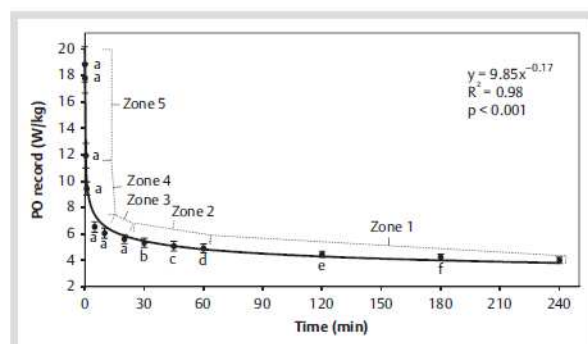
Fig. 1 Average RPP of the 17 cyclists. a significant difference between all record PO (p<0.05), b significant difference between all record PO except for 45' (p<0.05), c significant difference between all record PO except for 60' (p<0.05), d significant difference between all record PO except for 120' (p<0.05), e significant difference between all record PO except for 180' (p<0.05), f significant difference between all record PO except for 240' (p<0.05).
