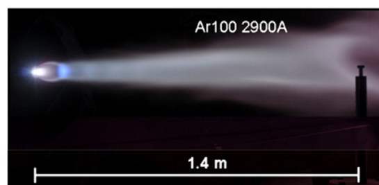
Figure 39: Photograph of PS-PVD plasma jets emitted from 03CP plasma torch. Chamber pressure and net power input were kept constant at 200 Pa and 60 kW [58]
