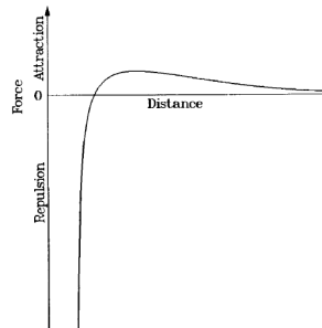
Figure 43: Intermolecular force field
