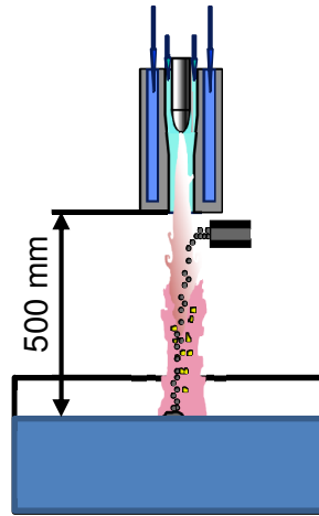
Figure 55: Schematic of the experiment to verify particle size evolution prediction. Water tank surface was equal to 0.2 \times 0.3 \text{ m}^2
