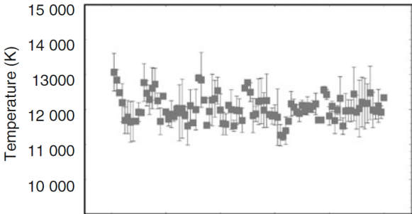
Figure 34: Hundred consecutive measurements of the peak temperature [18]
