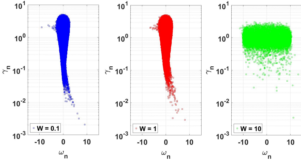
Figure 39 – Eigenvalues of the coupling matrix computed for N = 2000 atoms uniformly distributed in a cube of length L with a detuning of \delta = 0 and a resonant optical thickness of b_0 = 10 . 10 realizations on the distribution of the atoms are performed.
