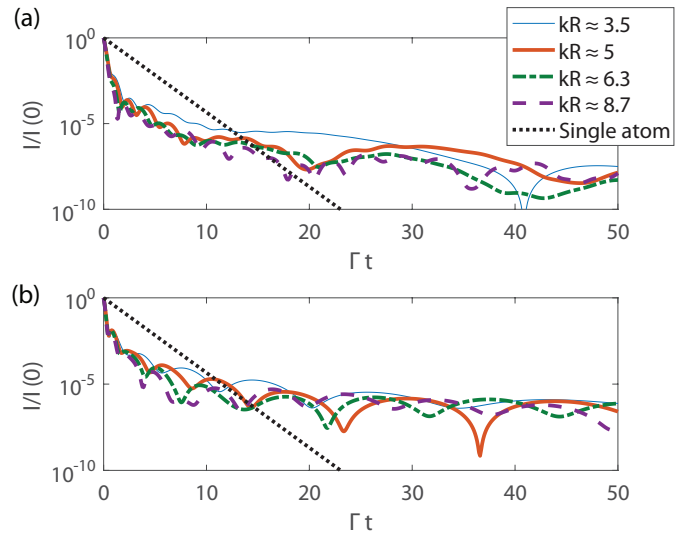
Figure 16 – Far-field intensity radiated in the forward direction, for a Gaussian cloud distribution with b_0 = 80 and driven far from resonance ( \delta = -10 ). Using the (a) Microscopic and (b) mean-field model.
