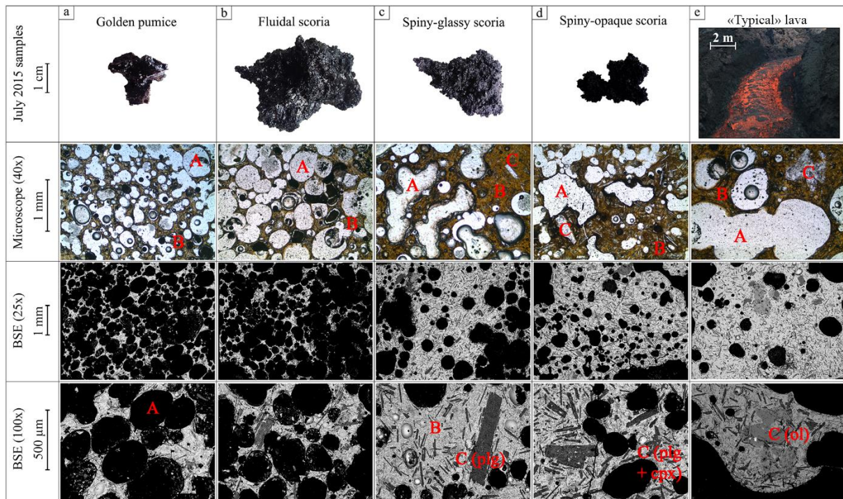
Figure 4.6 – General texture of the different July 2015 quenched samples: (a) golden pumice, (b) fluidal scoria, (c) spiny-glassy-scoria, (d) spiny-opaque scoria and (e) typical lava (sampled near the main vent). A is for vesicles, B for matrix (glass and microlites), C for micro-phenocrysts, plg for plagioclase, cpx for clinopyroxene and ol for olivine.
