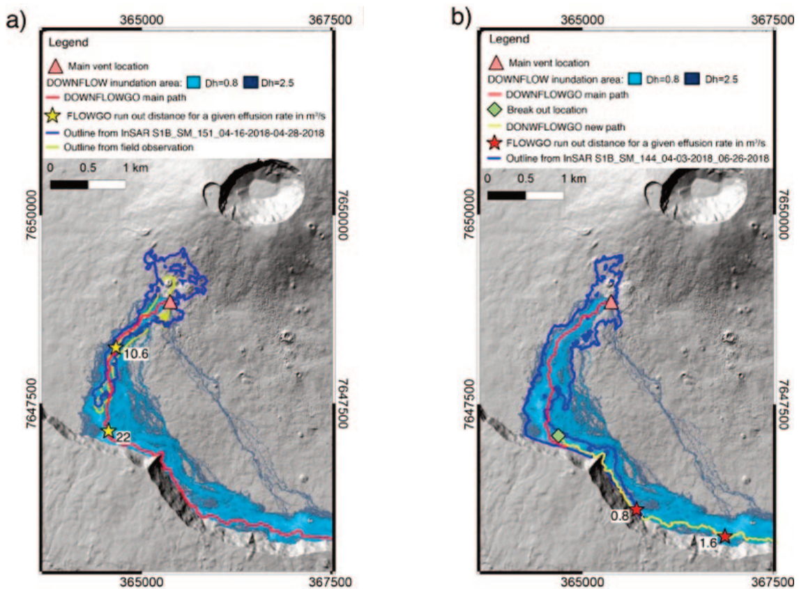
FIGURE 4. Distance down the LoSD (red line) that FLOWGO will run at the given effusion rates, these being the numbers (in \text{m}^3/\text{s} ) next to each star. Runs are given from (a) the initial vent location of 28 April, and (b) the tube exit on 9 May. Overlain are the limits of the flow field defined from InSAR incoherence (blue outline) and field mapping (yellow outline) on the same dates. Background shows the DOWNFLOW inundation area.
