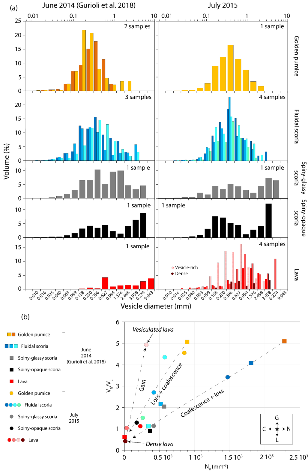
Figure 4.7 – (a) Vesicle Size Distributions (VSD) of the June 2014 (Gurioli et al. 2018) and July 2015 selected samples. (b) Vesicle to melt ratio ( V_G/V_L ) vs. vesicle density number ( N_V ). The different trends reflecting different mechanisms are represented by the arrows: N for bubble nucleation, G for bubble growth, C for bubble coalescence and L for bubble loss.
