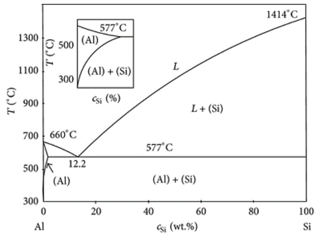
Figure 6.2: Al - Si phase diagram. Ref [127]
