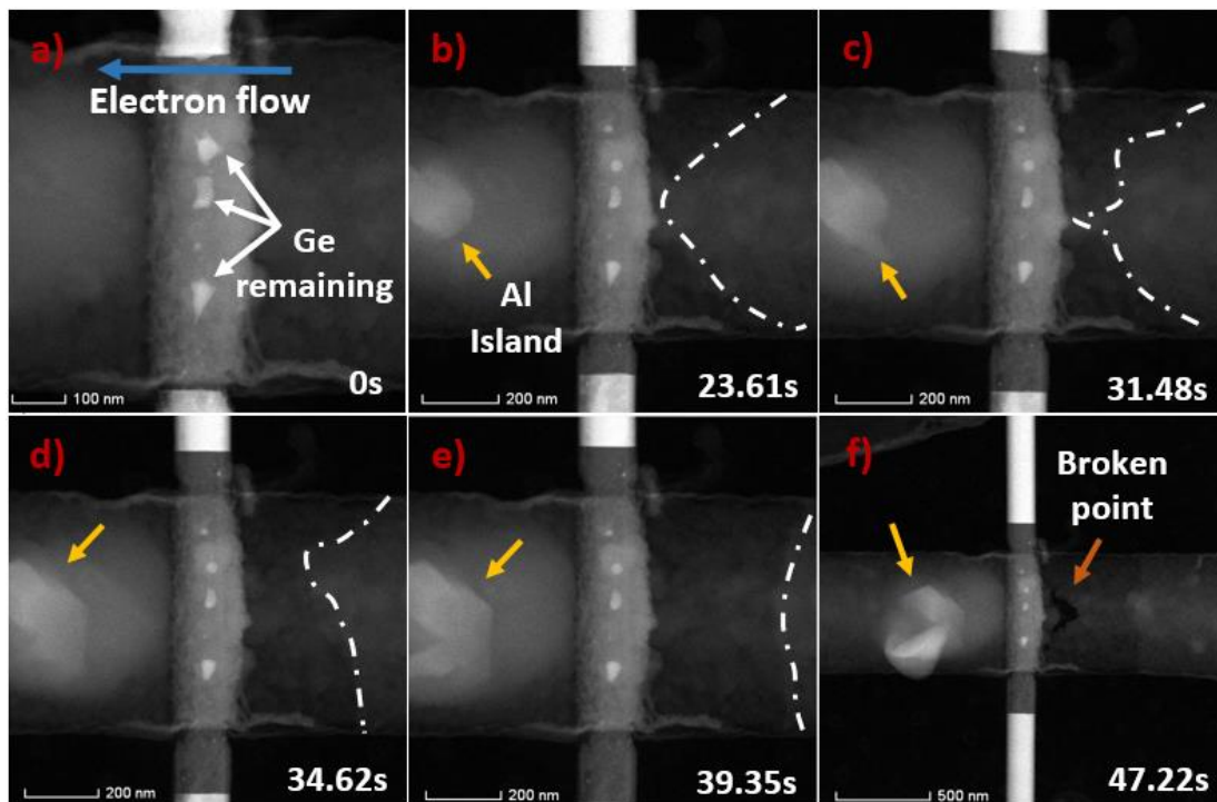
Figure 5.3: HAADF-STEM images of Al intruding in 130 nm Ge NW with 5 nm Al 2 O 3 shell by Joule heating method. a ) Some remaining Ge islands are present underneath the Al contact pad when the reacting front moved out. b-e ) The diffusion of Al atoms into the Ge NW and the formation of a large Al crystal (yellow arrows) lead to a local exhaustion of Al atoms on the contact pad. f ) A cracking point appeared on the right side of the NW in the Al contact, creating an open contact and blocking the heating current. The orange arrow indicates a broken point in the Al electrode. The scale bar varies in each image. See the supporting information SI M5.2.
