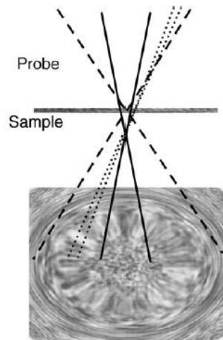
Figure 4.15: Schematic drawing of the Ronchigram formation at under-focus. Ref [95].
