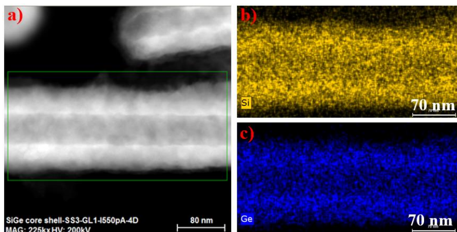
Figure A.6: (a) HAADF STEM image of a Si-Ge core shell NW before the thermal treatment of sample 2. The shell thickness is quite uniform with about 35 nm. (b-c) EDX mapping of the distribution of Si and Ge, showing the intermixing of both Si and Ge in the core and shell of the NW.
