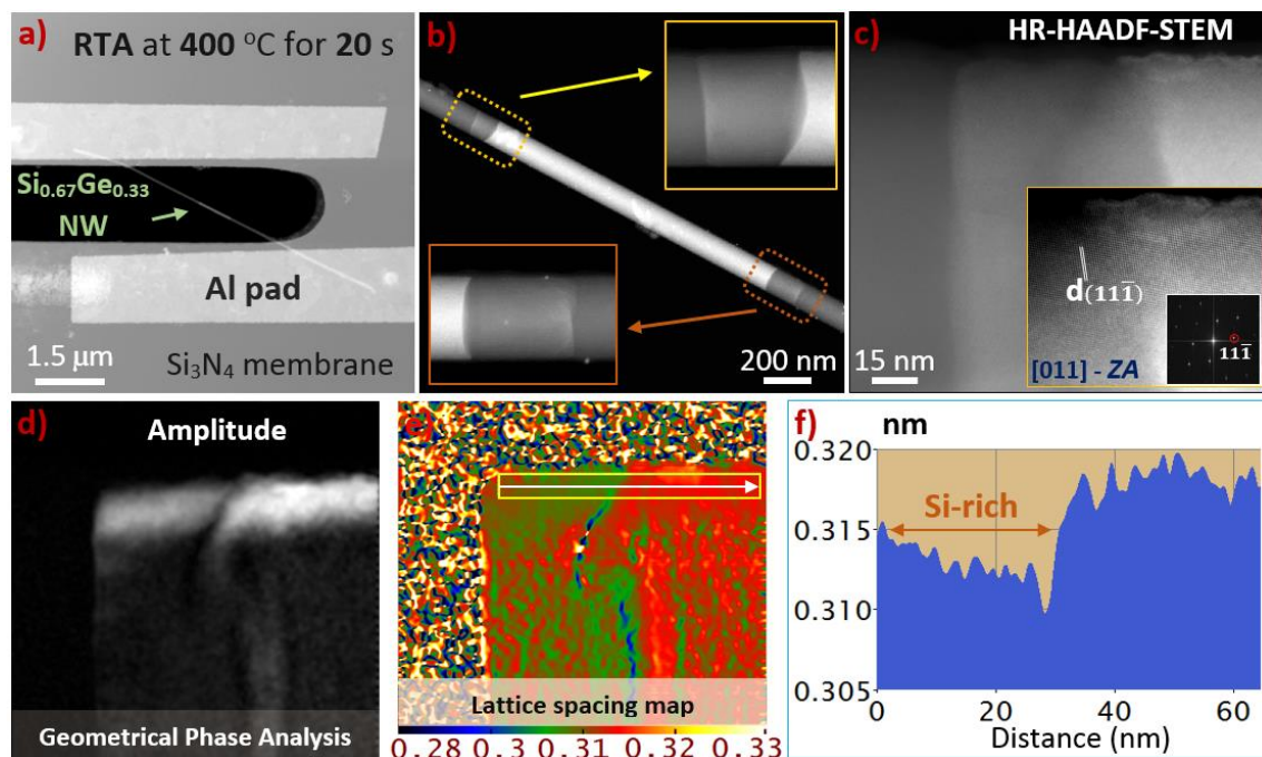
Figure 6.6: a ) HAADF STEM image of the Al contacted Si 0.67 Ge 0.33 NW crossing over the 2 μm x 8 μm hole on the 200 nm thick Si 3 N 4 membrane. b ) A zoom at the middle part of the NW showing the formation of the top and bottom double interface regions sandwiched between the reacted and unreacted part of the Si 0.67 Ge 0.33 NW. c ) The HR-HAADF-STEM image with zoom and corresponding FFT in the inset taken at the double interface on a different propagated NW, used for geometrical phase analysis (GPA). d-e ) The amplitude and lattice spacing map of the HR-
