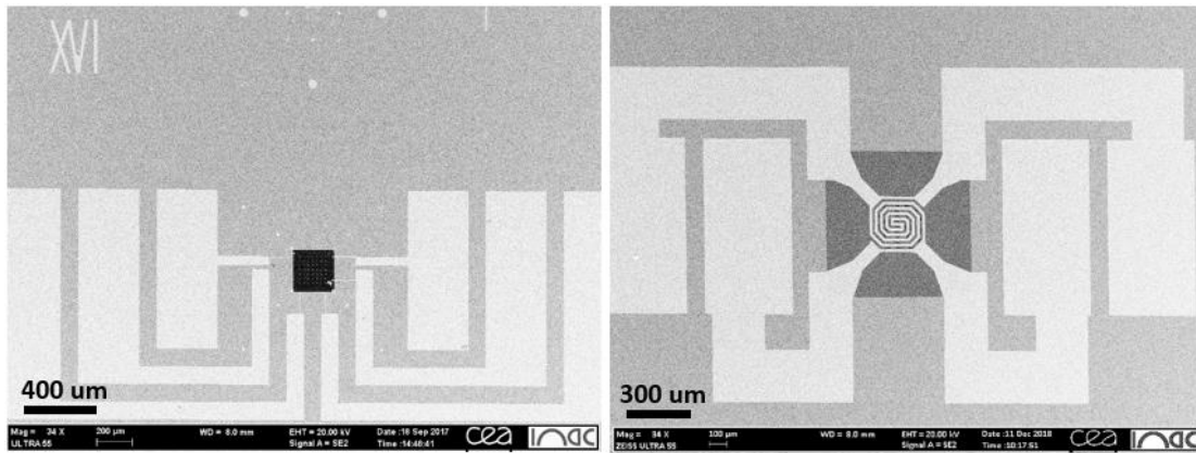
Figure 3.8: SEM images of (a) home-made 200 nm thick electron transparent \text{Si}_3\text{N}_4 membrane and (b) the temperature calibrated heater chips from DENSSolutions company.
