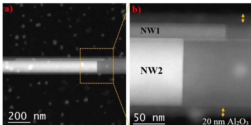
Figure 6.15: (a) HAADF STEM image of two propagated NWs with different diameters (30 and 108 nm) and (b) a zoom on the reaction interfaces showing the presence of sharp Si 0.67 Ge 0.33 interfaces.
