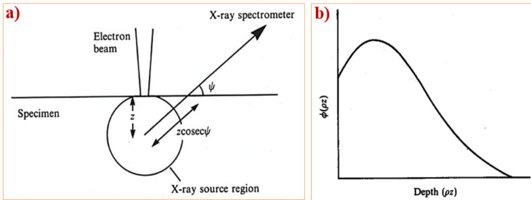
Figure 4.25: (a) Geometry of the X-ray absorption in a substance when being irradiated by an electron beam and (b) X-ray distribution as a function of depth z . \rho is the material density ( \text{g/cm}^3 ). Ref [102]
