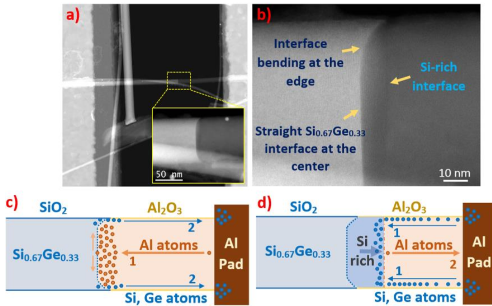
Figure 6.13: a) HAADF-STEM image of Al contacted \text{Si}_{0.67}\text{Ge}_{0.33} NW (83 nm in diameter) after being annealed at 400 °C for 20 s, 400 to 300 °C for 30 s and cooled down to room temperature during 4 min. The inset figure shows the zoom on the reaction interface having a convex shape. (b) The magnified image on the top part of the reaction interface showing a straight interface at the center and a bending shape at the NW edge. c-d) Schematic illustrations of Al, Si and Ge diffusion direction during the forward propagation of the \text{Si}_{0.67}\text{Ge}_{0.33} interface and backward diffusion of the Si-rich interface, respectively.
