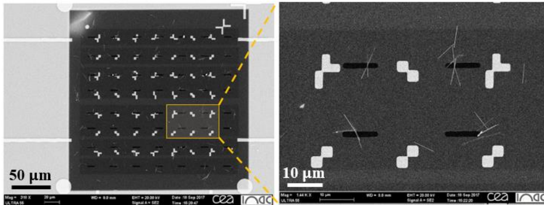
Figure 3.9: (a) SEM image of NW dispersion on the \text{Si}_3\text{N}_4 window and (b) a zoom on the yellow rectangular box showing the 2\ \mu\text{m} \times 8\ \mu\text{m} holes and markers with Ge NWs lying over the holes.
