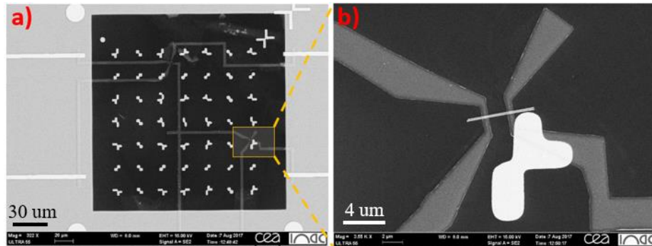
Figure 3.14: a) SEM image of the Al contacted n-doped Ge NWs on a 40 nm flat \text{Si}_3\text{N}_4 membrane and b) a zoom on the yellow rectangular box showing the Al pad contacted to the double Ge NWs.
