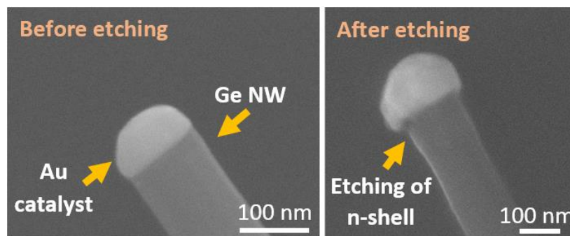
Figure 3.4: SEM images of the n-doped Ge NWs before and after the hydrogen peroxide ( H_2O_2 ) etching process. The etching process was done by dipping the sample in diluted H_2O_2 /DIW as ratio of 1:2 for 20 s and then DIW for 20 s, followed by N_2 gas blow. After the etching, about 20-30 nm of the n-doped shell was removed.
