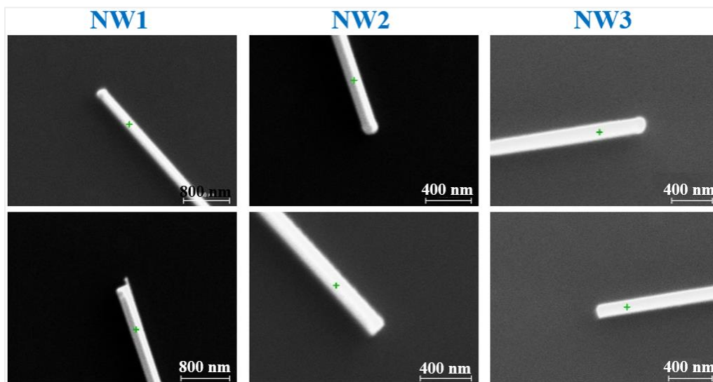
Figure 5.17: Positions of EDX point spectra analysis for the measurement of dopant concentration.
