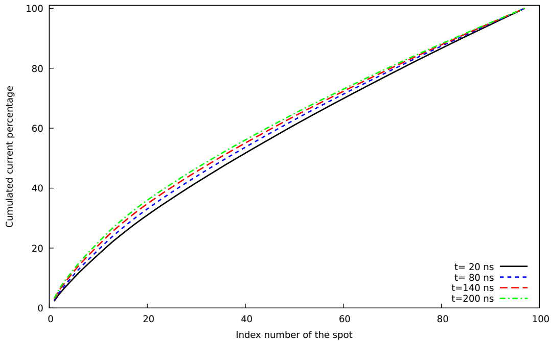
Figure 4.6: Cumulated current percentage in the a-pots sorted by decreasing size in a 0.1\text{ m}\Omega contact with constant tightening distance ( R_a = 12\text{ }\mu\text{m} , R_q = 4\text{ }\mu\text{m} ).
