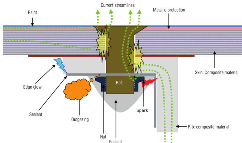
Figure 1.10: Schematic drawing of the different mechanisms that occur during sparking phenomenon. Taken from [29].
