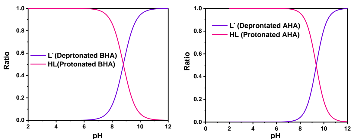
Figure II.14 Speciation diagrams of benzohydroxamic acid (left) in 0.1 M NaClO 4 at 25°C and acetohydroxamic acid (right) in 1.0 M NaCl at 25°C.
