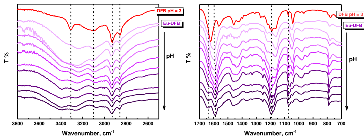
Figure IV.19 FTIR spectra of air-dried Eu(III)-DFB complexes as a function of pH (from 3.1 to 9.4). C_{\text{Eu(III)}} = C_{\text{DFB}} = 2.5 \times 10^{-2} \text{ M} at room temperature.
