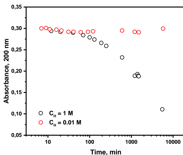
Figure A. 7 Variation of UV absorbance of 1 \times 10^{-5} M DFB solution at 200 nm as function of time.
