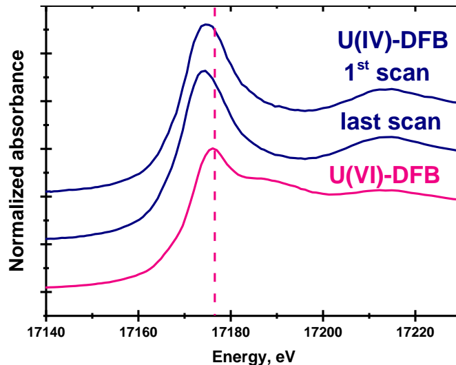
Supplementary figure for page 102: XANES spectra of U(IV)-DFB and U(VI)-DFB complexes.
