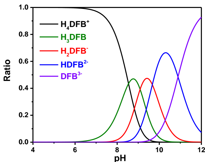
Figure II.12 Speciation diagram of desferrioxamine B ( I = 0.7 M Na, \text{HClO}_4 , T = 25 °C).
