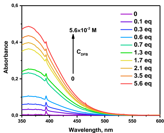
Figure IV.10 Absorption spectra of Eu(III) at 10^{-2} M with increasing amount of DFB at pH = 3.7 (left) and 4.5 (right) (I = 0.5 M, 0 \leq C_{\text{DFB}} \leq 5.6 \times 10^{-2} M).
