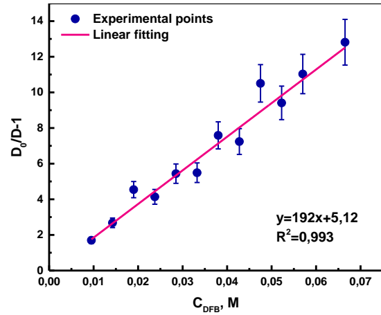
Figure IV.4 Variations of D_0/D-1 as function of DFB concentration ( C_{Acetate} = 5 \times 10^{-3} M, I = 0.7 M (Na, HClO_4 ), T = 25^\circ C , pC_H = 4.75 ).
