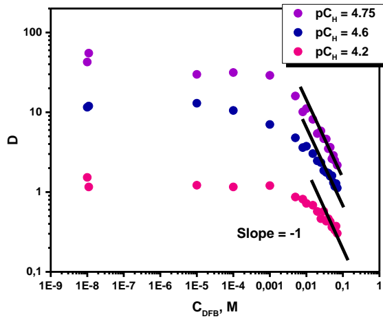
Figure IV.3 Variations of D as function of DFB concentration at different pC_H ( C_{TTA} = 2.5 \times 10^{-2} M, I = 0.7 M (Na, HClO_4 ), T = 25^\circ C , C_{Acetate} = 5 \times 10^{-3} M).
