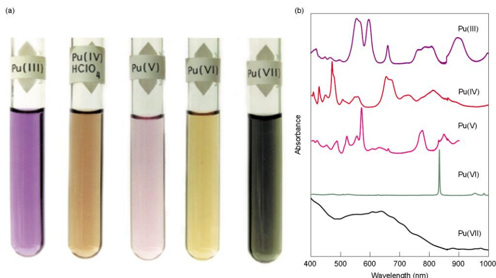
Figure II.7 (a) The color of non-complexed plutonium at various oxidation states in 1 M HClO 4 from Pu(III) to Pu(VI) and in strong base for Pu(VII) (b) their corresponding absorption spectra [2000CLA].
