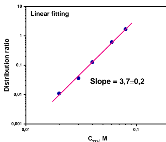
Figure IV.21 Variations of the distribution ratio D of ^{227}\text{Th} as function of total TTA concentration in toluene ( I = 0.7 \text{ M} ( \text{Na}, \text{HClO}_4 ), pC_H = 1.0 , T = 25^\circ\text{C} ).
