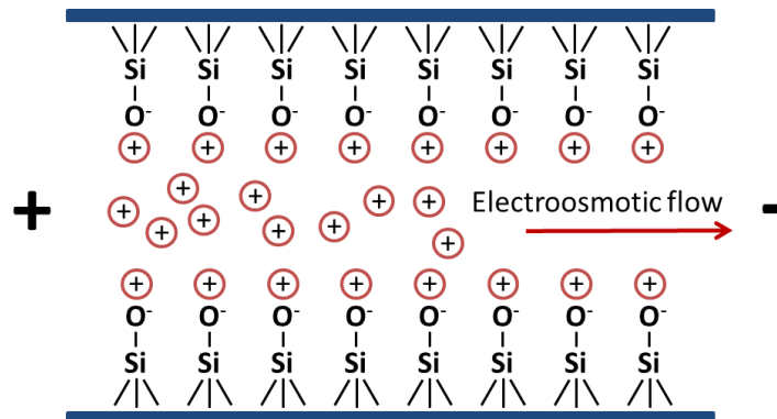
Figure III.2 Schematic of electroosmotic flow.
