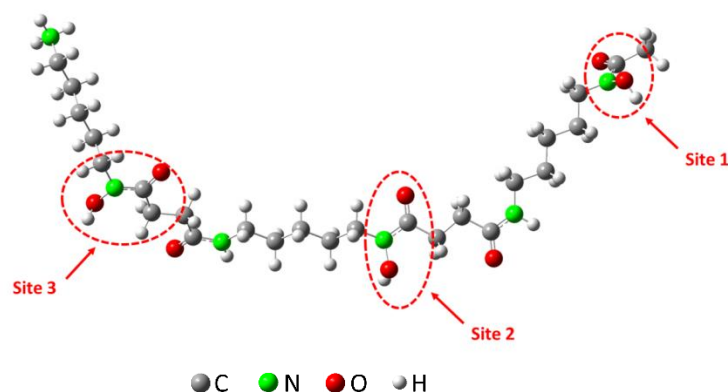
Figure IV.33 Optimized structure of ligand DFB.
