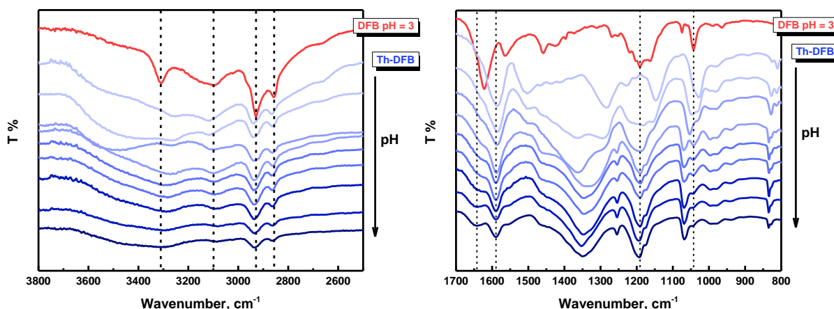
Figure IV.32 FTIR spectra of the air-dried Th(IV)-DFB complexes as a function of pH (from 1.3 to 9.1) C_{\text{Th(IV)}} = C_{\text{DFB}} = 2.5 \times 10^{-2} \text{ M} at room temperature.
