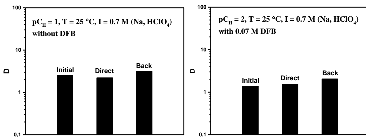
Figure A. 4 Values of D in the back and direct extraction of Th(IV) at pC_H = 1 , I = 0.7 M (Na, \text{HClO}_4 ) without DFB (left) and at pC_H = 2 , I = 0.7 M (Na, \text{HClO}_4 ) with 0.07 M DFB (right).
