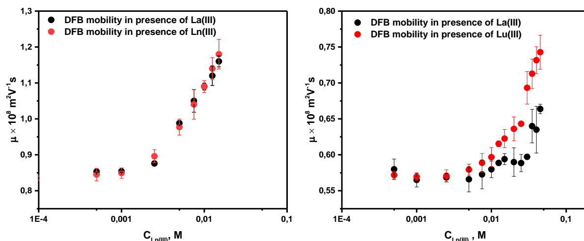
Figure IV.14 Mobility of 1 \times 10^{-4} M DFB as function of La(III) (black points) and Lu(III) (red points) at I = 0.1 M (left) and 0.5 M (right) pH = 2.5, T = 25 °C.
