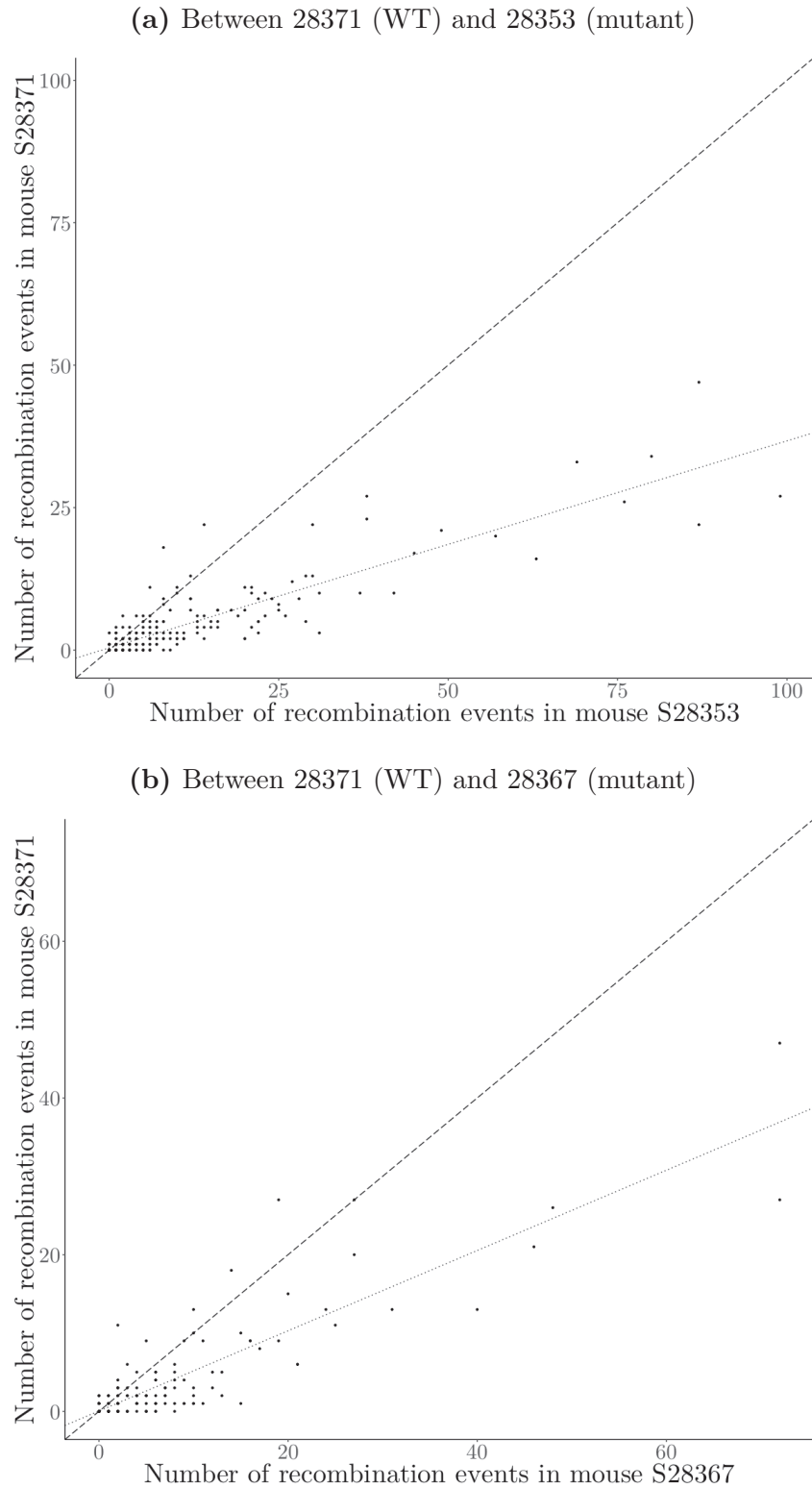
Figure A.6: Correlation of the number of recombination events in shared hotspots between the 28371 WT mouse and the two mutant mice.
