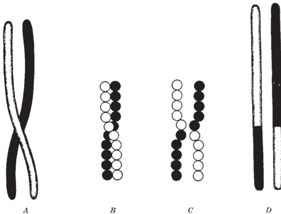
Figure 1.2: Original drawing of crossing over in The Mechanism of Mendelian Heredity (Morgan et al., 1915).
