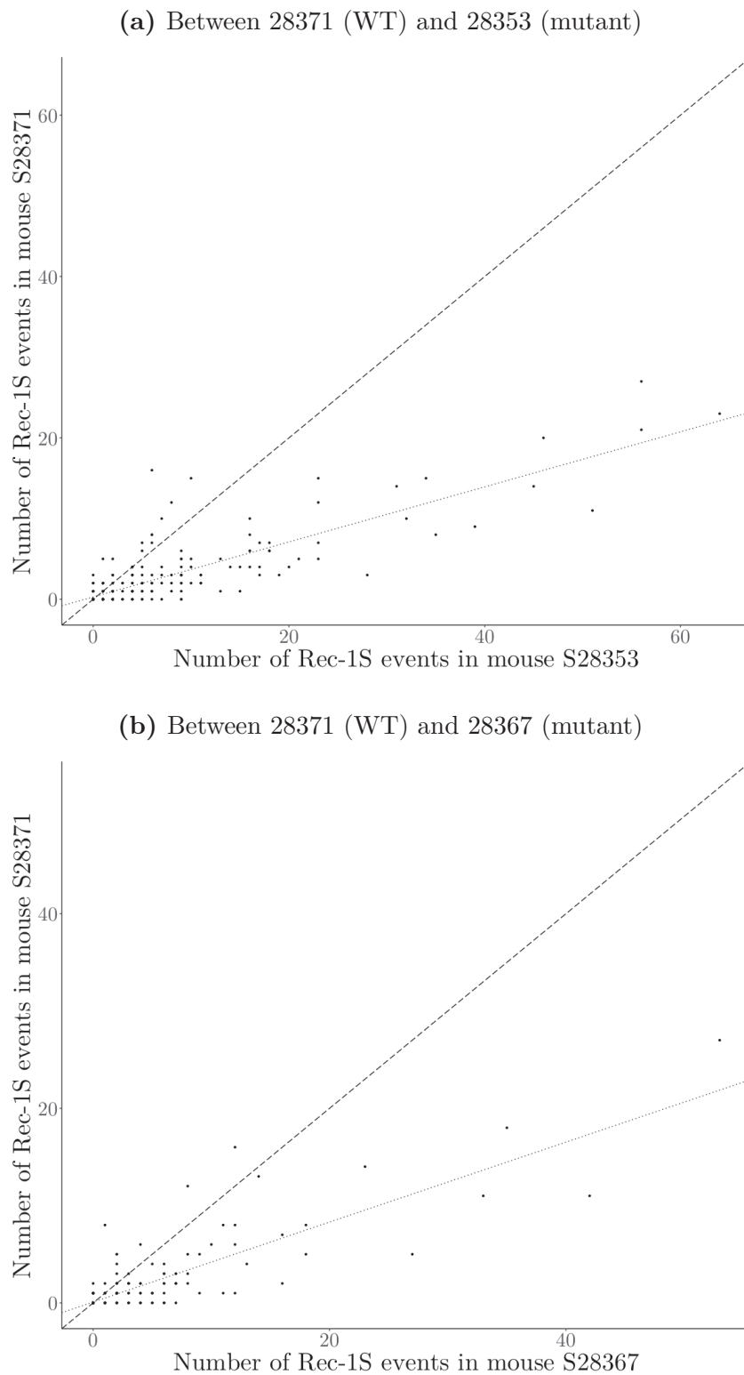
Figure A.9: Correlation of the number of Rec-1S events in shared hotspots between the 28371 WT mouse and the two mutant mice.
