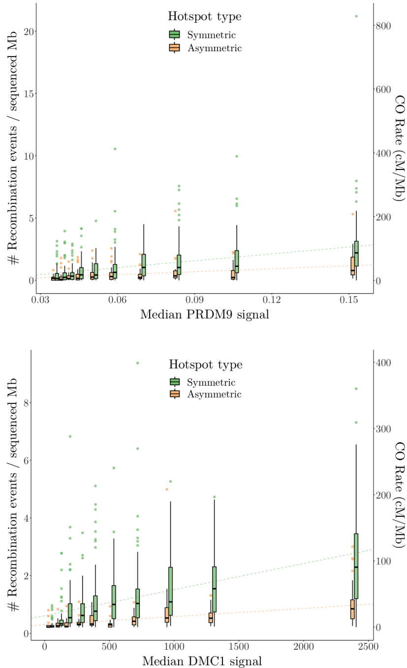
Figure 6.3: Asymmetric hotspots display lower recombinational activity than expected by their PRDM9 (top) or DMC1 (bottom) binding affinity.
