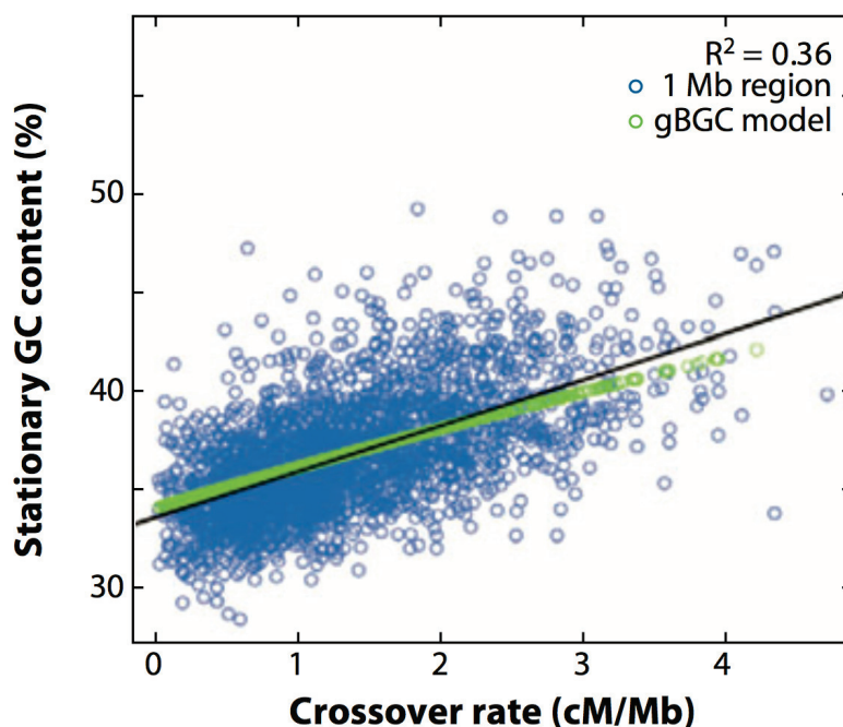
Figure 4.3: Correlation between the stationary GC-content ( GC^* ) and the crossover rate (cM/Mb) in human autosomes.
