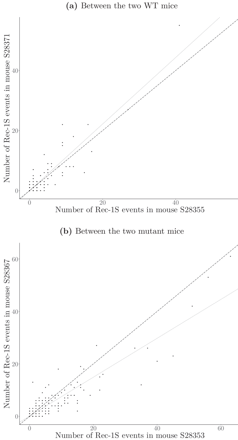
Figure A.8: Correlation of the number of Rec-1S events in shared hotspots for the two WT (a) and the two mutant (b) mice.
