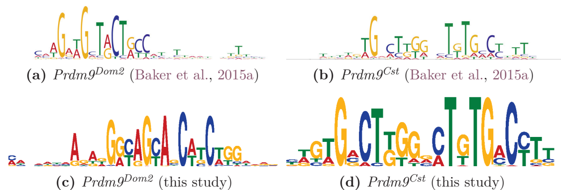
Figure 7.1: Comparison of consensus motifs for Prdm9 Dom2 and Prdm9 Cst . The consensus motifs for Prdm9 Dom2 (left) and Prdm9 Cst (right) alleles found by Baker et al. (2015a) are reported at the top and those found in our study at the bottom.
