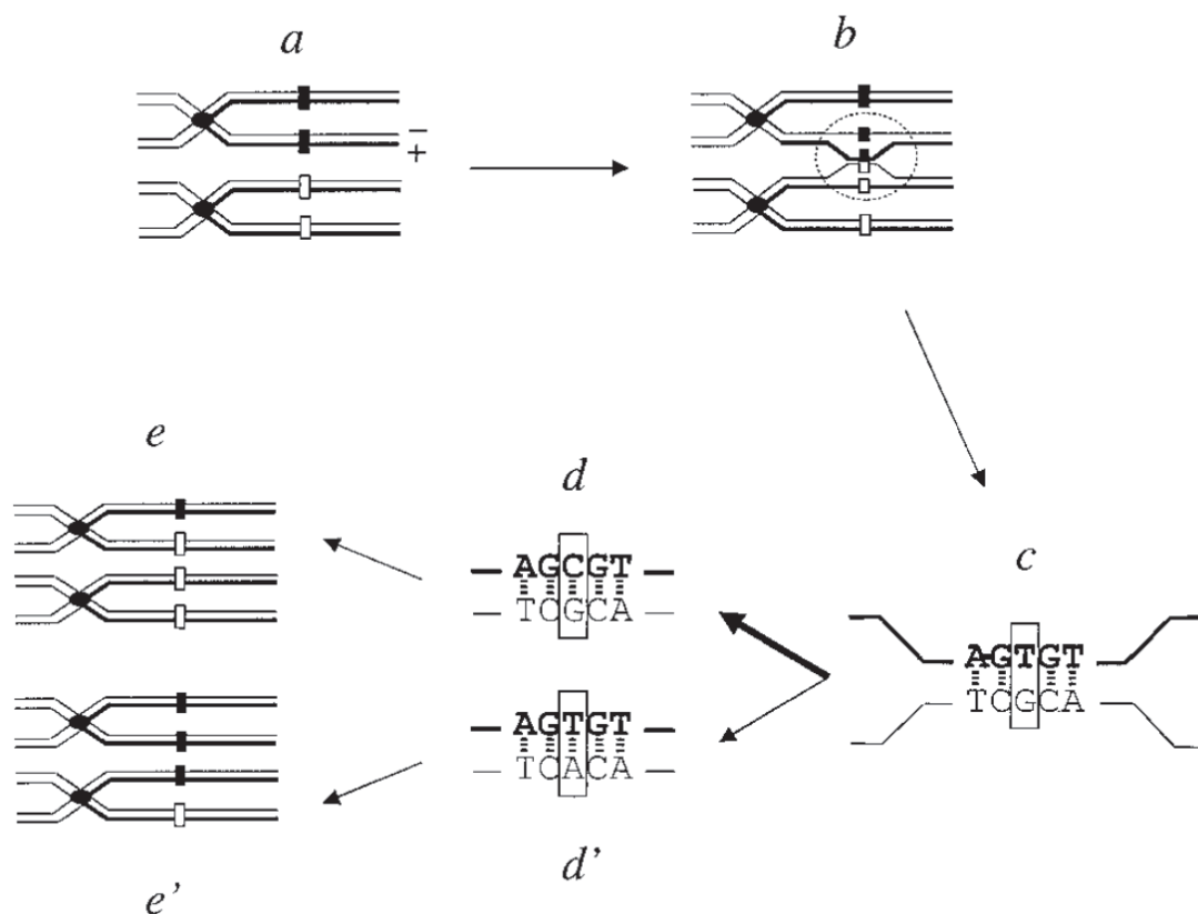
Figure 4.2: Gene conversion during a recombination event involving a strong (G or C) versus a weak (A or T) base mismatch.
