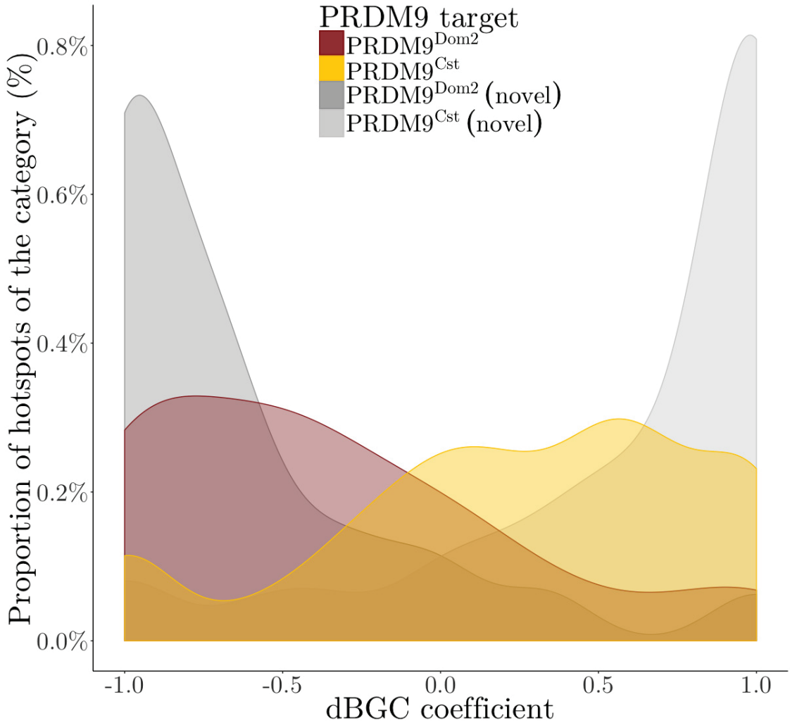
Figure 7.3: Distribution of the dBGC coefficient across categories of hotspots. The dBGC coefficient ( b_{dBGC} ) was directly extrapolated from the observed frequency of CAST-donor fragments in the pool of gametes ( x ) as follows: b_{dBGC} = 2 \times x - 1 (Nagylaki, 1983) (see main text). The distribution was reported for four groups of hotspots: those targeted by PRDM9 Dom2 which were either completely eroded (NOV.tB.chB, dark grey) or not (tB.chB and tB.sym, red) in the B6 lineage, and those targeted by PRDM9 Cst which were either completely eroded (NOV.tC.chC, light grey) or not (tC.chC and tC.sym, yellow) in the CAST lineage. The frequencies were normalised to the total number of hotspots in each category.
