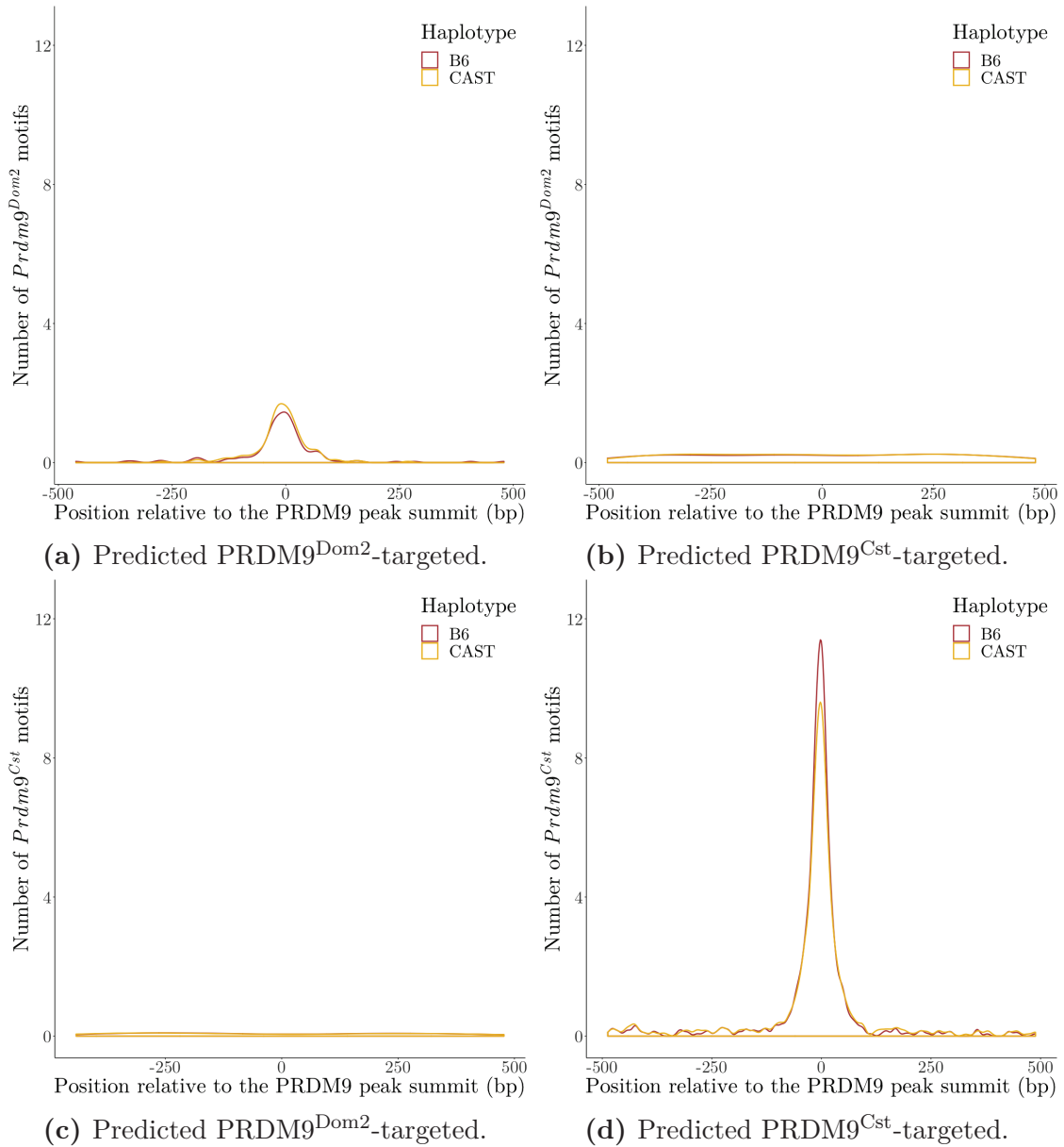
Figure 7.2: Occurrences of Prdm9^{Dom2} and Prdm9^{Cst} consensus motifs along hotspots predicted to be targeted by these alleles.
