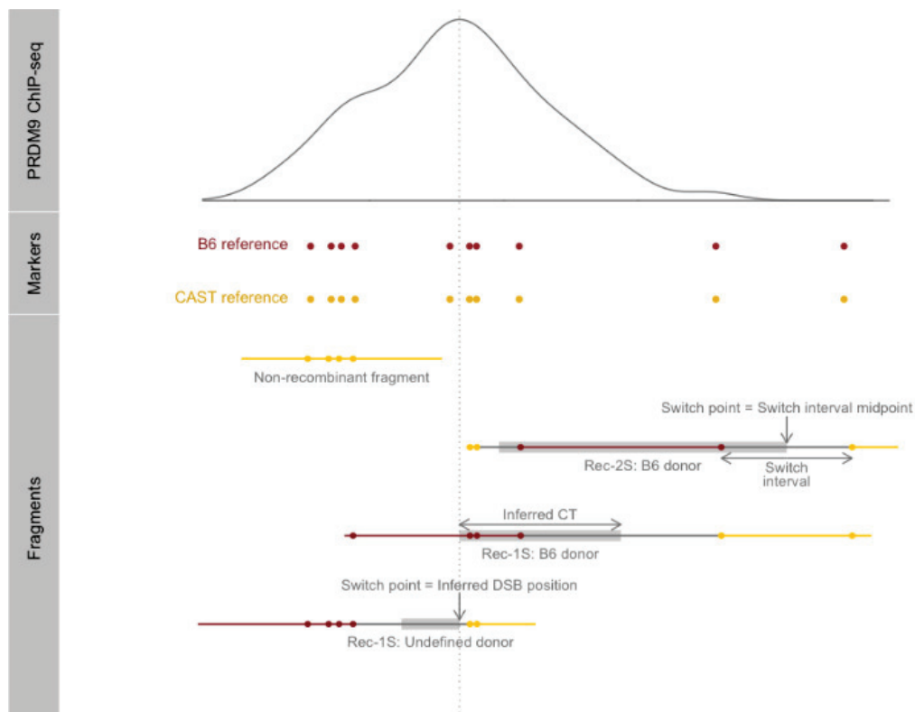
Figure 6.4: Terminology used to characterise recombination events.
