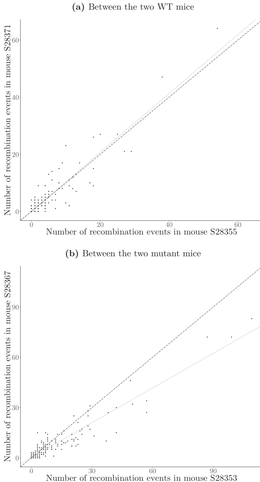
Figure 8.3: Correlation of the number of recombination events in shared hotspots for the two WT (a) and the two mutant (b) mice.
