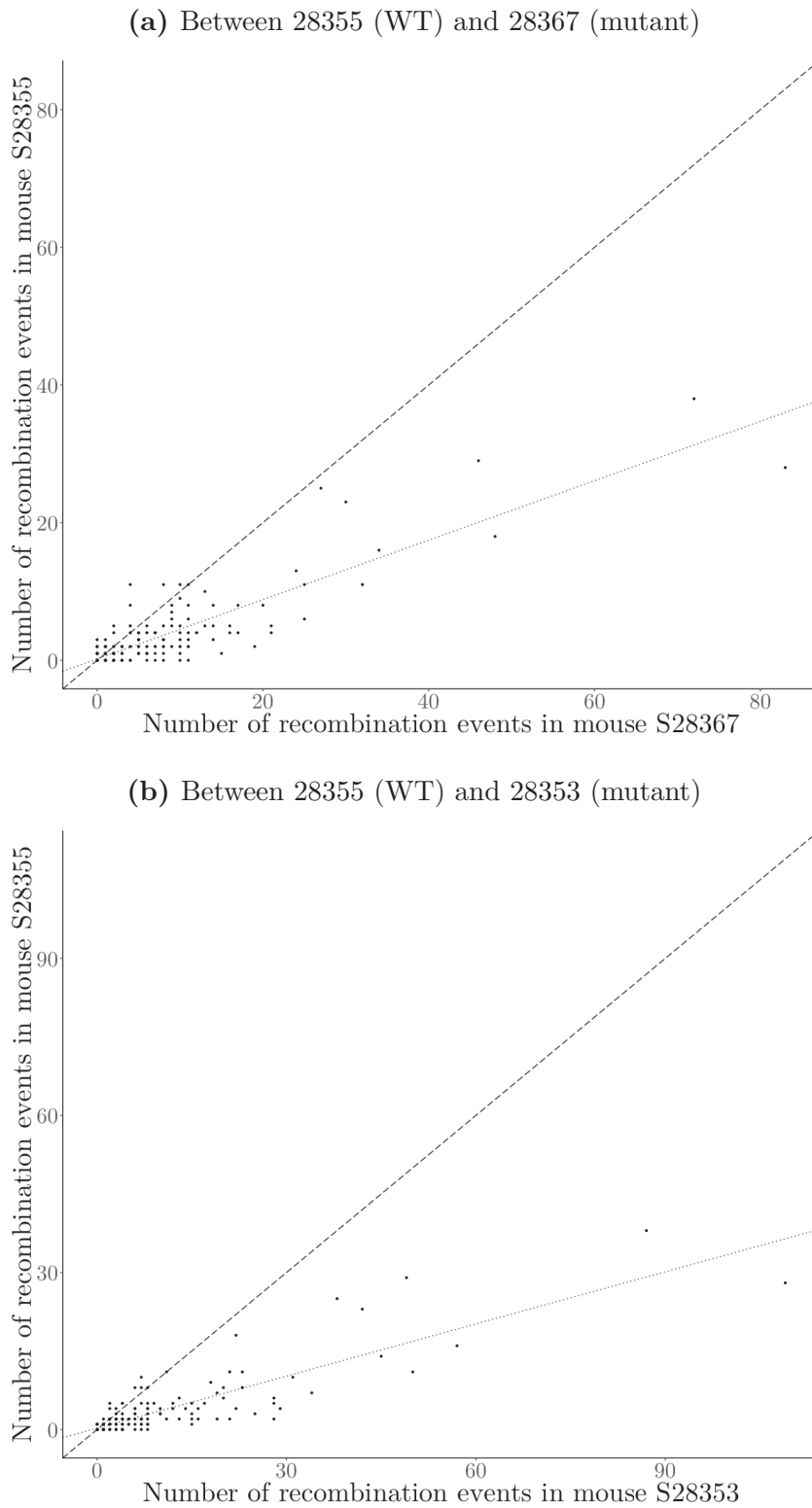
Figure A.7: Correlation of the number of recombination events in shared hotspots between the 28355 WT mouse and the two mutant mice.
