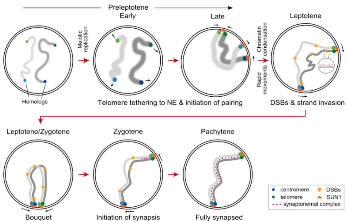
Figure 2.3: Mouse preleptotene DSB-independent pairing model proposed by Boateng et al. (2013).
