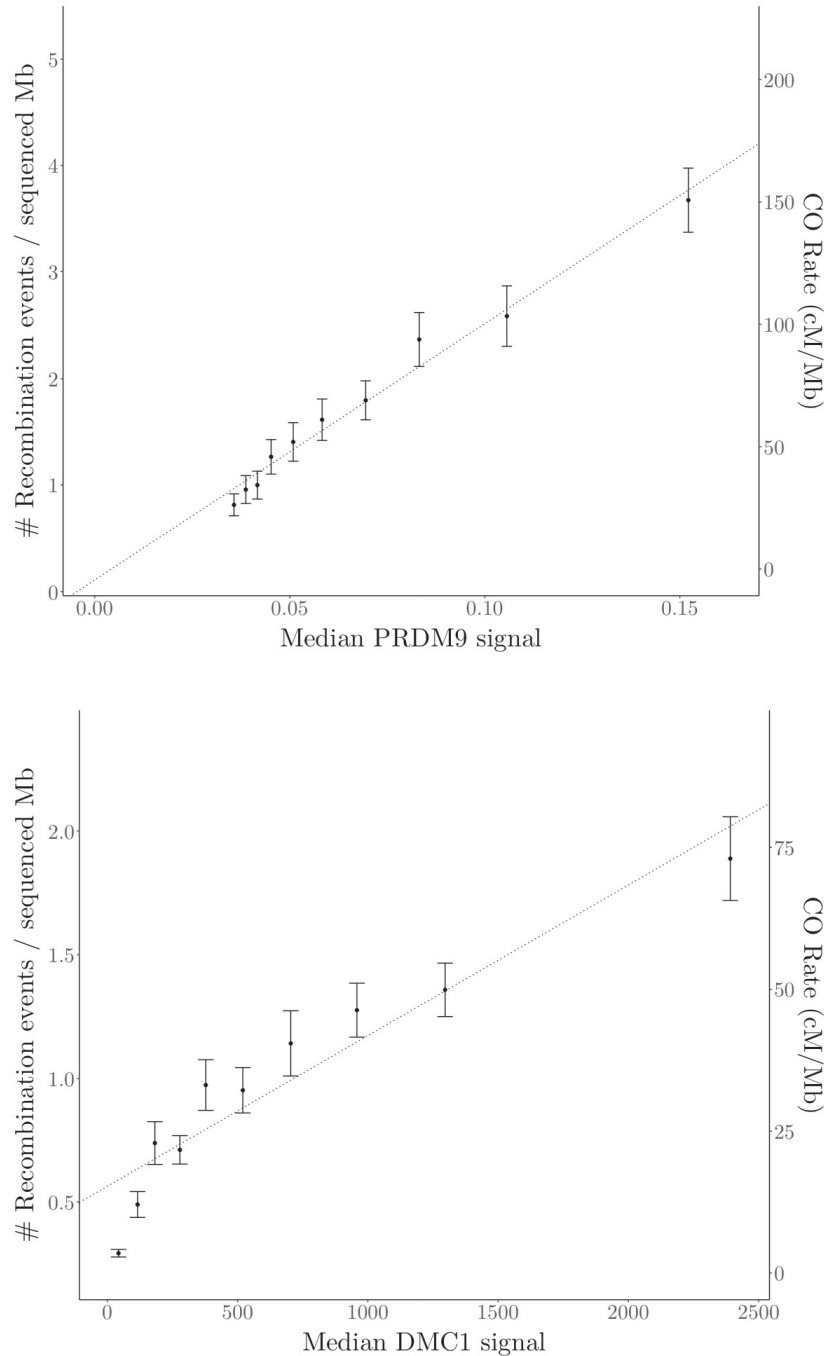
Figure 6.2: Proportionality between the recombination rate and either PRDM9 (top) or DMC1 (bottom) binding intensity.
