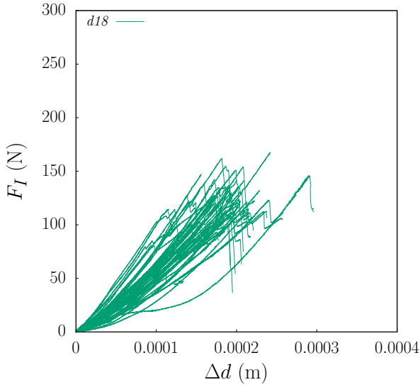
Figure 3.12 : Diametrical load vs. vertical displacement curves resulting from radial compression test performed on two sizes: a – d18 (combining MP1 and MP2) and b – d20 (see Figure 3.6 ).
