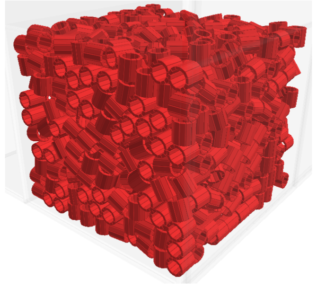
Figure 6.13 : A sample with a geometry of true prism – P_19×17_d_01_A (see Appendix B ). The base is a square with a side size of 19 cm. The sample contained 1 000 shells d18-S1 .
