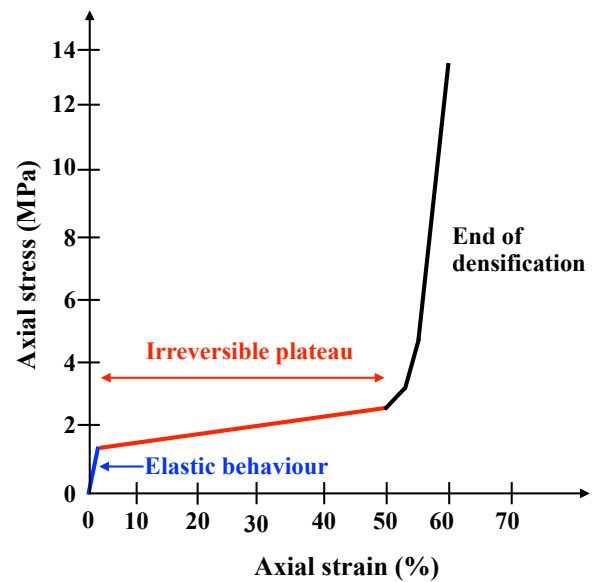
Figure 1.4 : Typical mechanical response of compressible layer (coated shells) obtained from uniaxial compression.
