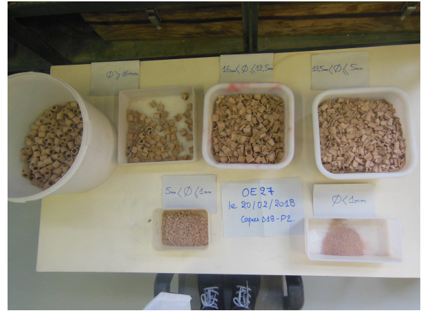
Figure 6.5 : The oedometer test finished at \sigma_n = 0.42 MPa ( Figure 6.4 ): a – A view of the top surface after the test (in contact with the loading plate), and b – The fragments divided into the sieve sizes ( Figure 6.6 ).
