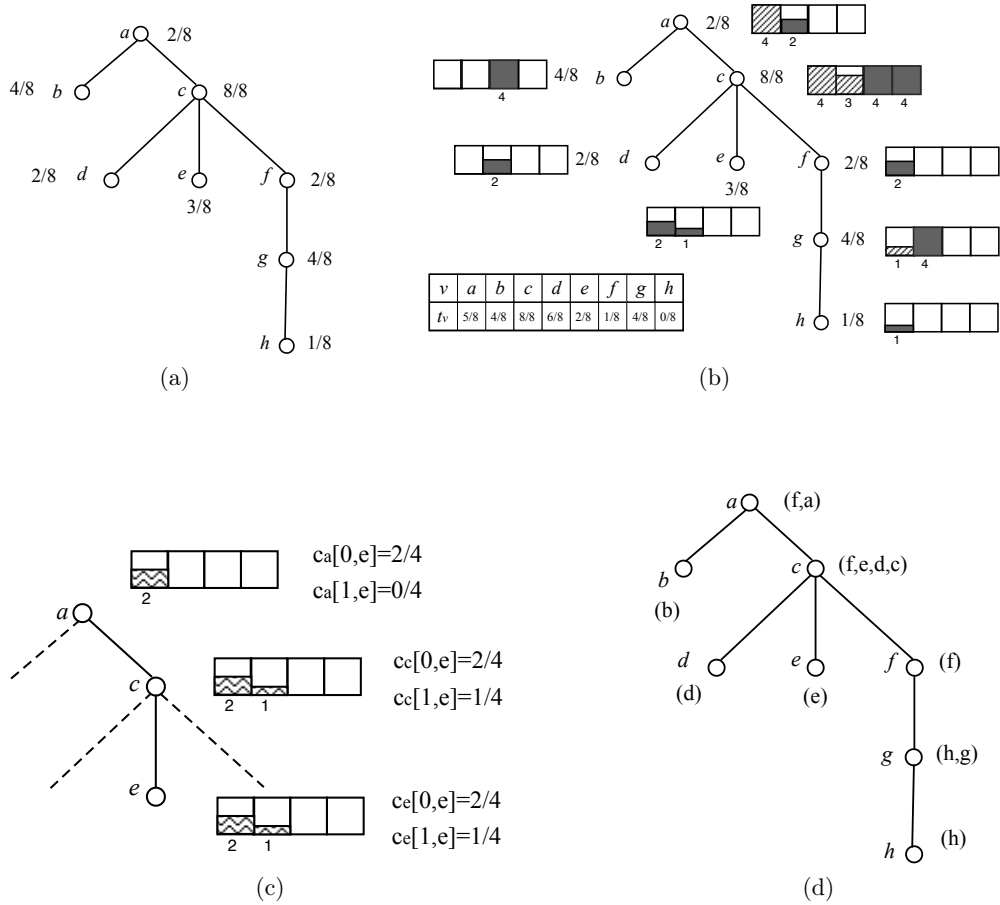
Figure 3.2: Illustration of Algorithm 2 and 3. The depicted tree T' has vertex set V = \{a, b, c, d, e, f, g, h\} and vertex weights: \frac{v}{w'(v)} \begin{array}{c|c|c|c|c|c|c|c|c} a & b & c & d & e & f & g & h \\ \hline \frac{2}{8} & \frac{4}{8} & \frac{8}{8} & \frac{2}{8} & \frac{3}{8} & \frac{2}{8} & \frac{4}{8} & \frac{1}{8} \end{array}
