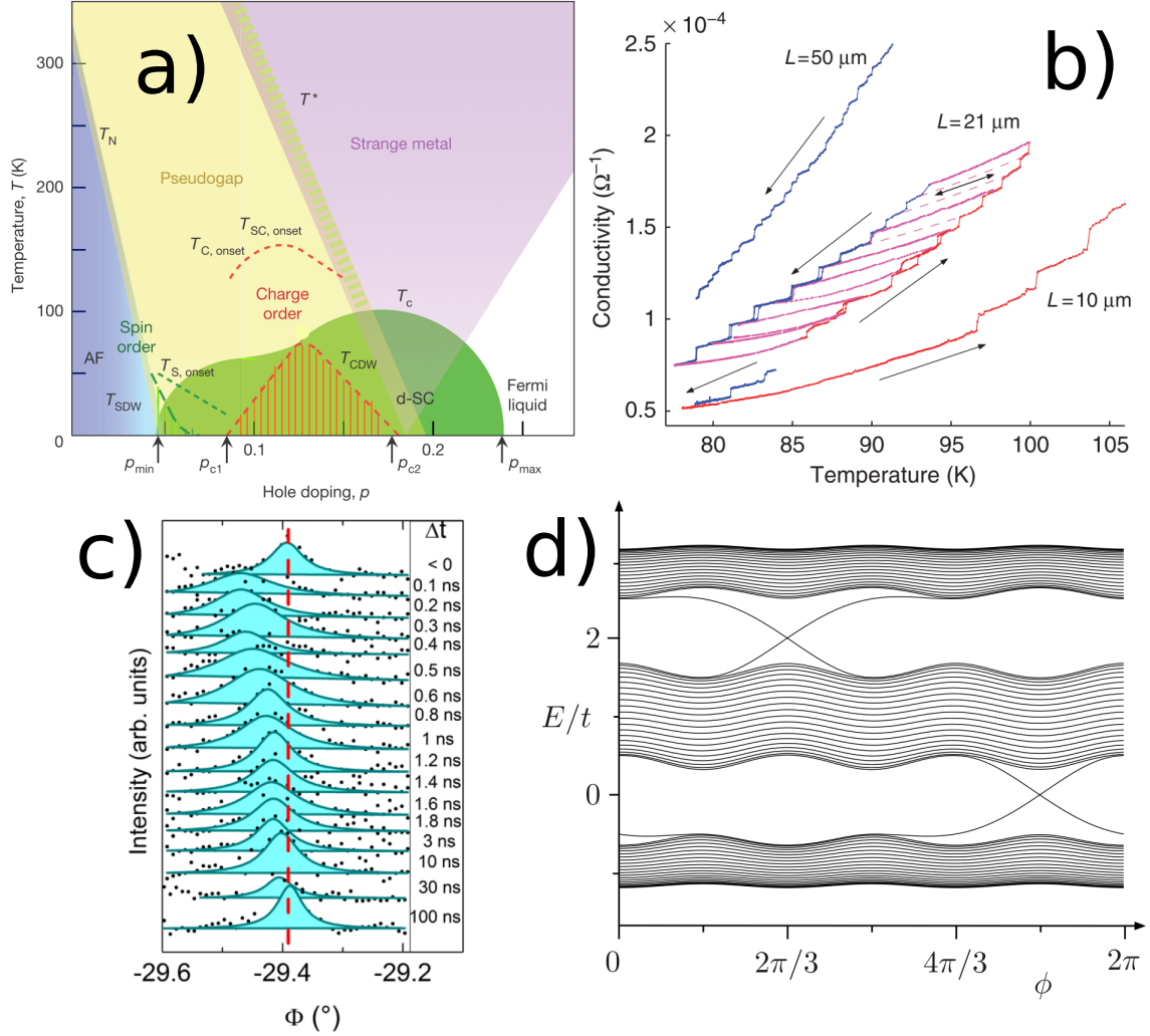
Figure 1.8: a) Cuprate phase diagram showing a CDW order at low temperature for hole doping p_{c1} < p < p_{c2} [35]. b) Quantized conductivity in K_{0.3}MoO_3 [36]. c) Time resolved CDW relaxation observed in pump probe X-ray diffraction in chromium [15]. d) Topological ingap edge states in a 1D CDW model [37].
