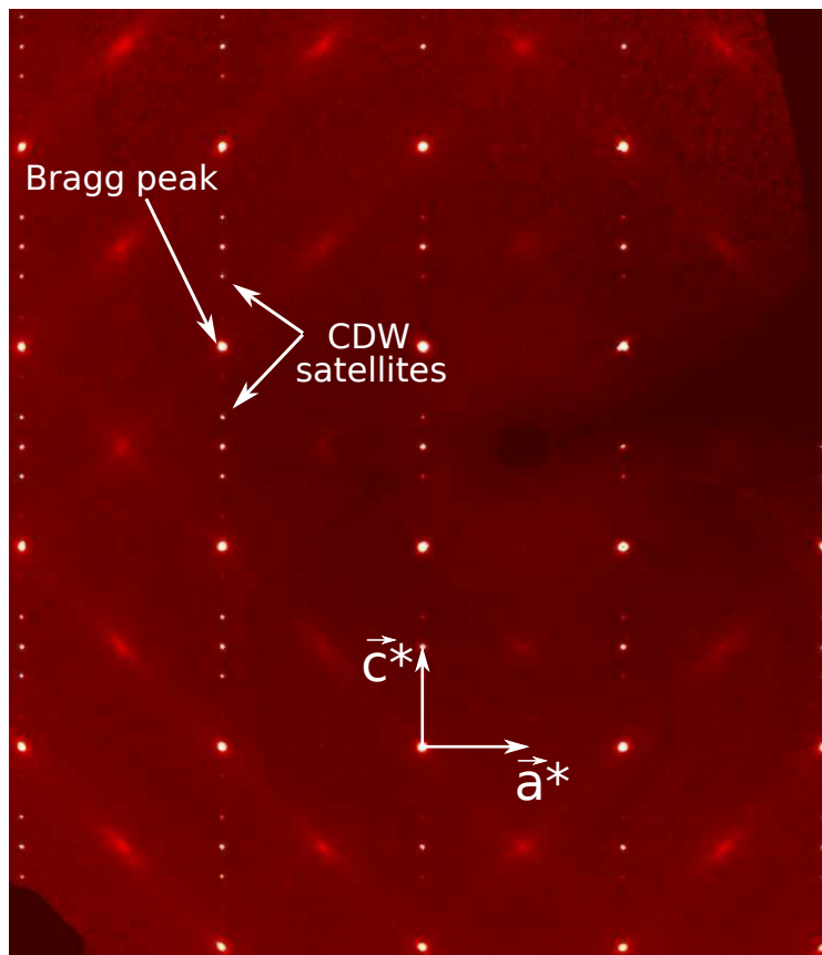
Figure 2.9: Diffraction of \text{TbTe}_3 at 300K performed on the 4 circles diffractometer of Cristal beamline at synchrotron SOLEIL. The CDW is along \vec{c}^* and the satellite are visible at \pm q_{cdw} around several Bragg peaks.
