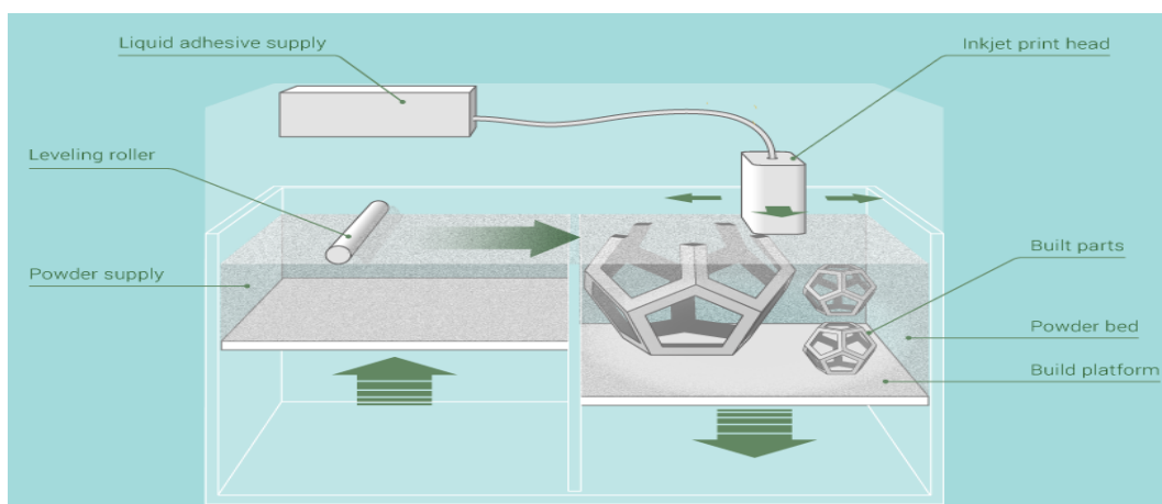
Figure I-36- Binder Jetting [31]
