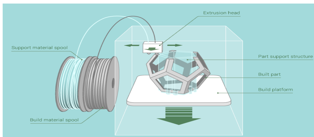
Figure I-38- Fused Deposition Modeling [31]
