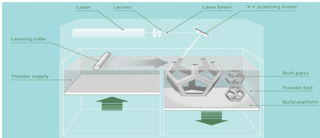
Figure I-37 - Laser sintering [31]
