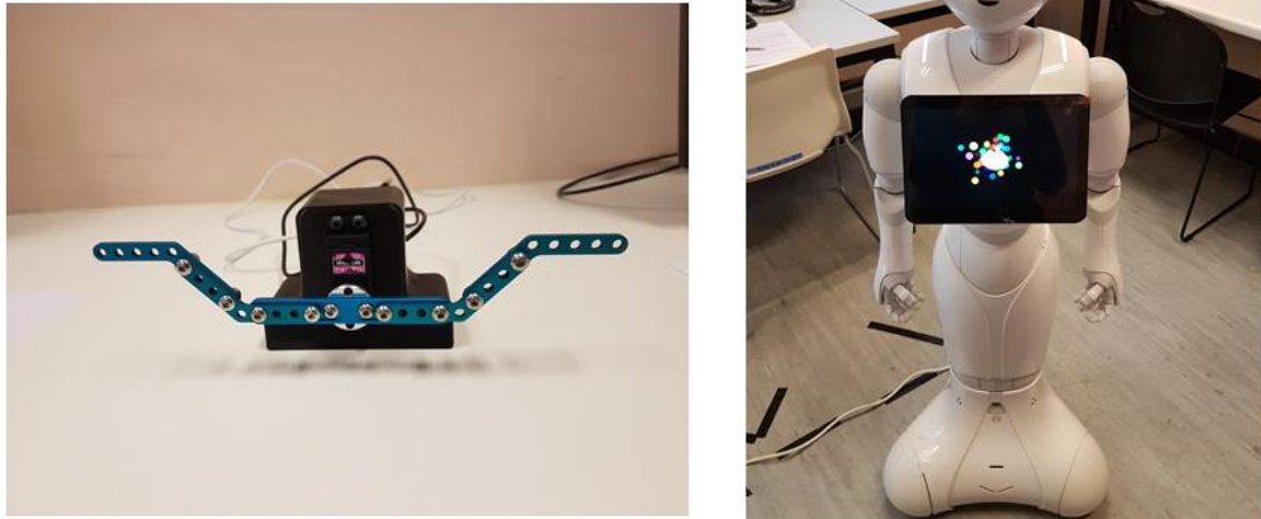
Figure 19. Illustration of the two types of robots used during the experiment. The servomotor (on the left) could execute a keypress with the left or right metallic arm. The humanoid robot, Pepper, (on the right) could perform a keypress with the left or right fist.
