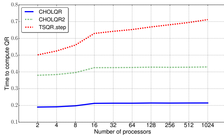
Figure 6.5 – Weak scaling
