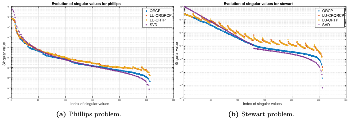
Figure 4.4 – Evolution of the singular values computed by QRCP, LU-CRQRCP, and LU-CRTP, compared to the SVD, for different problems.
