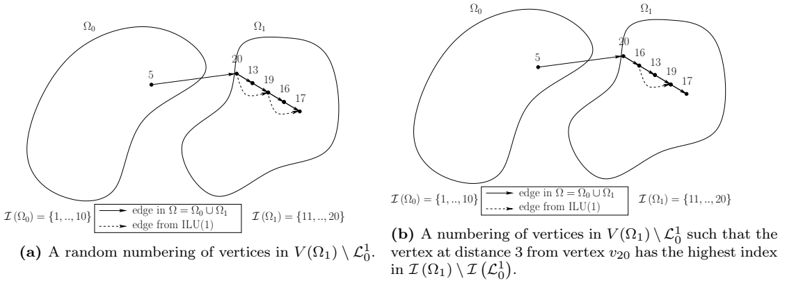
Figure 3.2 – Impact of the numbering of the vertices in subdomain \Omega_1 on the CA-ILU(k) overlap with k = 1 . A vertex is represented by a point and an oriented edge by an arrow. The number above each vertex is its index in \mathcal{I}(\Omega) . Consider a matrix A of size 20 and its associated graph \Omega partitioned into 2 subdomains \Omega_0 and \Omega_1 having a set of indices \mathcal{I}(\Omega_0) and \mathcal{I}(\Omega_1) , respectively. Subdomain \Omega_1 has \mathcal{L}_0^1 = \{v_{20}\} numbered with the highest number in \mathcal{I}(\Omega_1) . Subfigures differ in the way they number the vertex at distance 3 from the boundary layer. In 3.2a, this vertex is not numbered with the highest index of \mathcal{I}(\Omega_1) \setminus \mathcal{I}(\mathcal{L}_0^1) . In 3.2b, this vertex has the highest number of \mathcal{I}(\Omega_1) \setminus \mathcal{I}(\mathcal{L}_0^1) .
