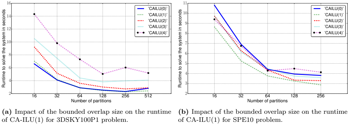
Figure 3.29 – Comparison of the runtime of CA-ILU(1) when the overlap size is bounded by \eta = \tau \times \frac{n}{p} where n is the size of the matrix, p the number of subdomains and \tau = 2 . The number of subdomain increases from 16 to 512. GMRES is set with a maximum of 3000 iterations, a restart of 200, and a relative tolerance of 1e - 6 .
