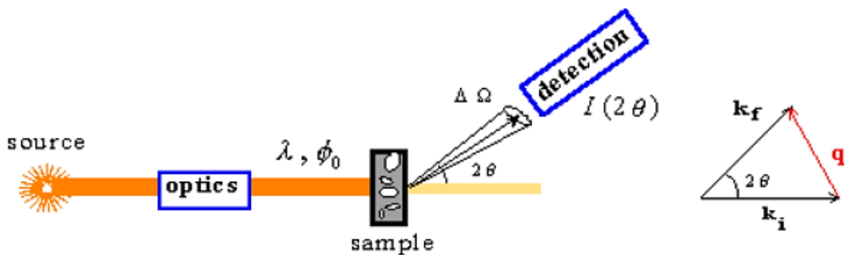
Figure 2. 9. Schematic view of a typical scattering experiment.
