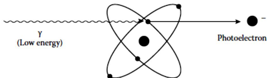
Figure 1. 12. Photoelectric effect [68].
