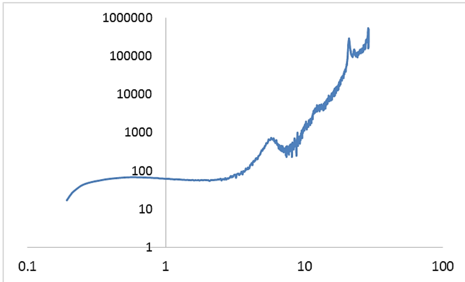
Figure V. 5. The plot of \ln(q) and \ln(I_{Abs}q^4)
