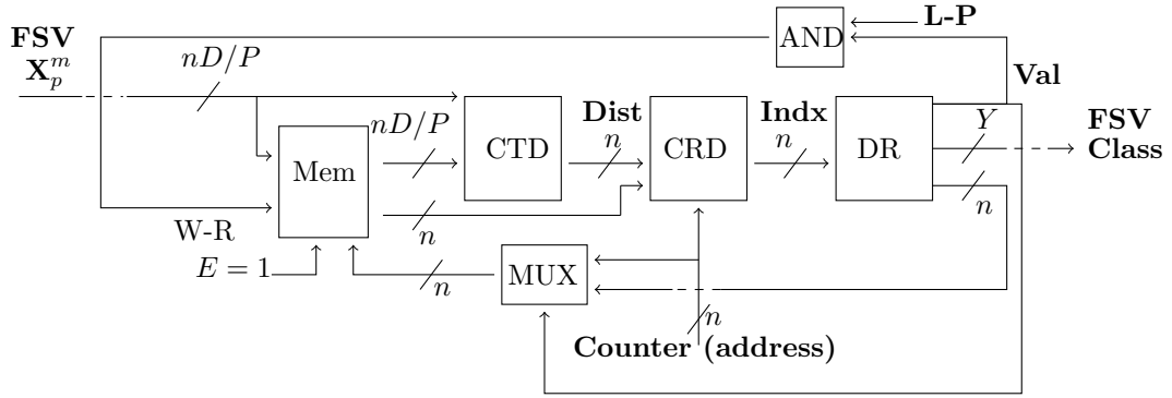
Figure 4.7: Hardware architecture of Processing block. Note that “FSV” refers to feature subvector, “Mem” refers to Memory, “CDT” refers to Compute Distance, “CRD” refers to Compare Distance and “DR” to Distance Register.
