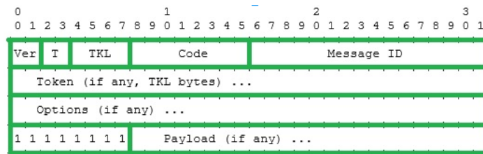
Figure A.4 – CoAP Message Format.
