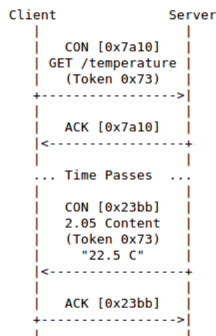
Figure 3.6 – Separate Response
