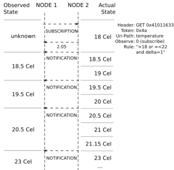
Figure 3.12 – CoAP2 subscription experiment
