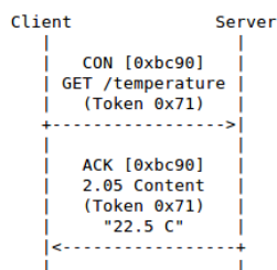
Figure 3.5 – Piggybacked Response
