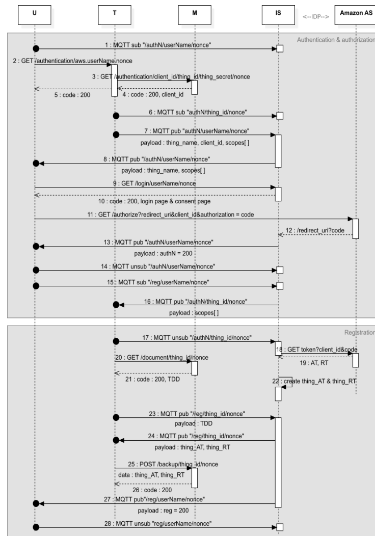
Figure 2.7 – Sequence diagram of the implementation
