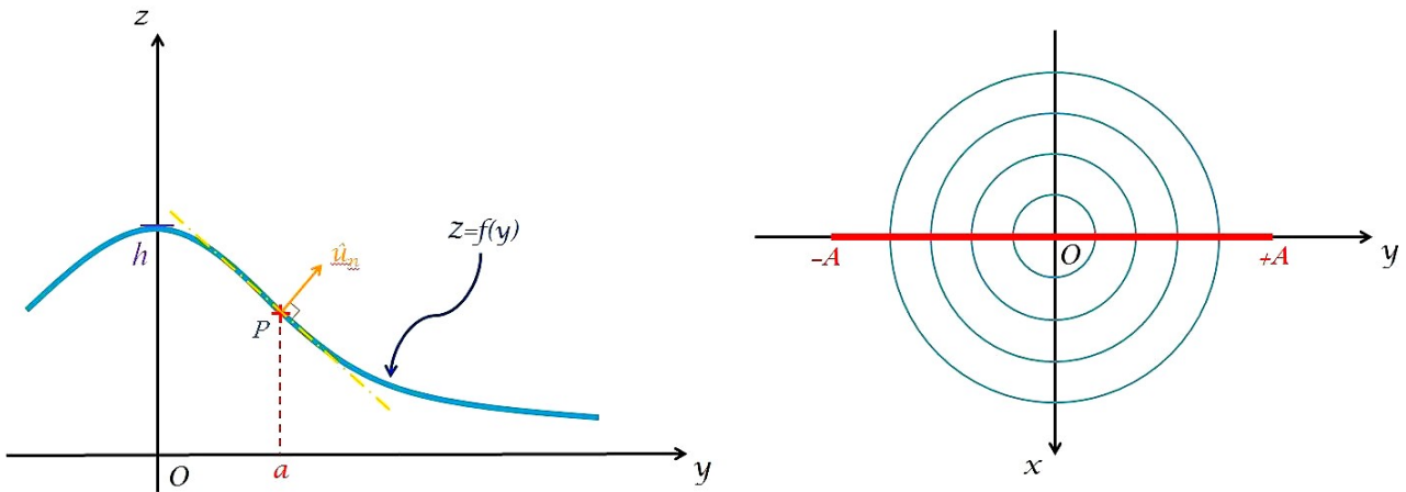
Figure E.5: Geometry of the deformation profile. (Left figure) Side view of the axisymmetric bump-like deformation of the interface. \hat{u}_n is the unit vector normal to the deformation profile z = f(y) at point P(0, a, f(a)) . (Right figure) Top view of the hydraulic bump. Each circle corresponds to a set of points located at a given altitude z .
