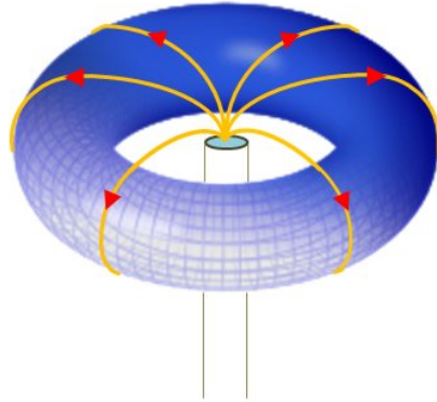
Figure 2.8: Schematic view of the axisymmetric base state. Our tiny subaquatic fountain generates a toroidal flow in its vicinity.
