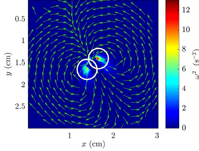
Figure 2.23: Typical interfacial vorticity field. For convenience, the square of the vorticity \omega^2 is plotted rather than vorticity itself. This way we handle only positive values, whereas vorticity is an algebraic quantity. The vector field is the one of the velocity map shown above, save that here all vectors have the same length normalised to unity so as to make the dipolar pattern more visible. The centres of the white circles coincide with the maxima of vorticity.
