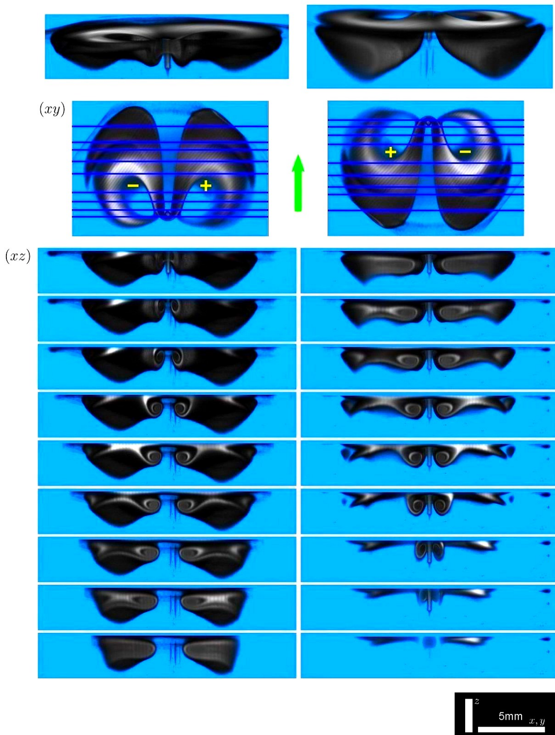
Figure 2.18: Peeling the coloured cloud. Series of back (resp. front) ‘cut views’ shown in column on the left (resp. right). (xy) denotes the horizontal plane of the top views and (xz) the vertical plane of the back/front views. Successive positions of the cut plane marked by blue lines. Volume ‘peeled’ in the direction of the arrow. The perspective views in the header of the plate give a global insight of the cloud shape. To ensure good visibility, each voxel is rescaled to a size \delta x \delta y \delta z = (34.26 \times 34.26 \times 68.52) \mu\text{m}^3 by imposing an aspect ratio \delta z/\delta x = 2 instead of the initial 1.3 value and performing a zoom that multiplies all lengths by 1.52. The yellow + (resp. -) sign denotes clockwise (resp. anticlockwise) vortex rotation.
