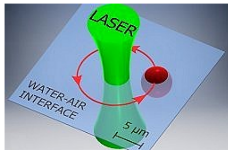
Figure 2: Closed orbital track of a light-absorbing microsphere around the centre of an optical trap. We use tiny particles about 5\ \mu\text{m} in diameter. Ibid.
