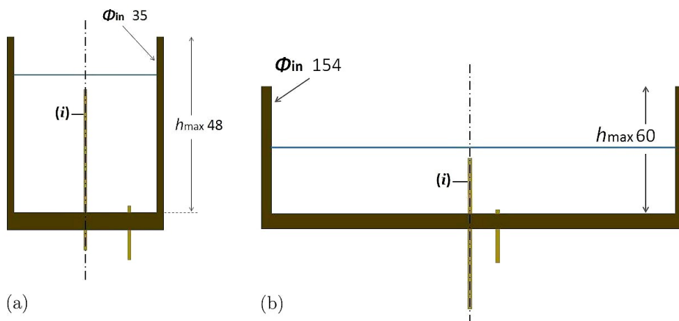
Figure A.1: Dimensions of the small (a) and large (b) cells (not to scale). Diameters and heights expressed in mm. The injection nozzle (i) has an inner diameter \varnothing_{\text{inj}}^{\text{in}} 0.55 mm.
