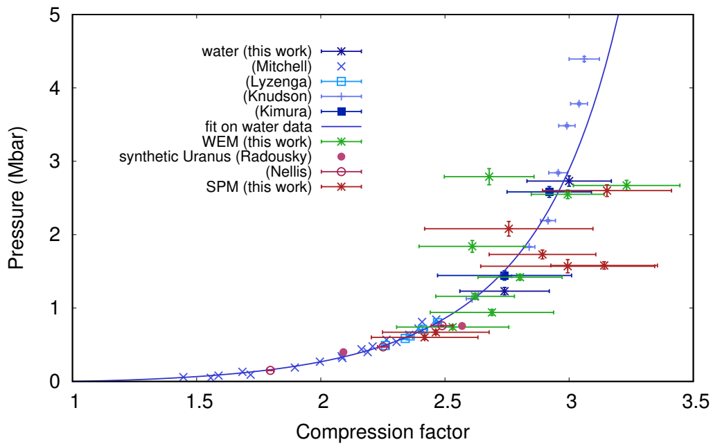
Figure 4.8 – Pressure as a function of the compression factor ( \rho/\rho_0 ) along the Hugoniot curve of water, WEM, and SPM. Our data are relative to the state created immediately after the shock has entered the sample. Previous data for water [Mitchell and Nellis (1982); Lyzenga et al. (1982); Knudson et al. (2012); Kimura et al. (2015)] and for “synthetic Uranus” [Radousky et al. (1990); Nellis et al. (1997)] are also shown. The transposition on the P-\rho/\rho_0 plane of a linear fit on the U_s - U_p data from Knudson et al. (2012) is provided as a guide for the eye.
