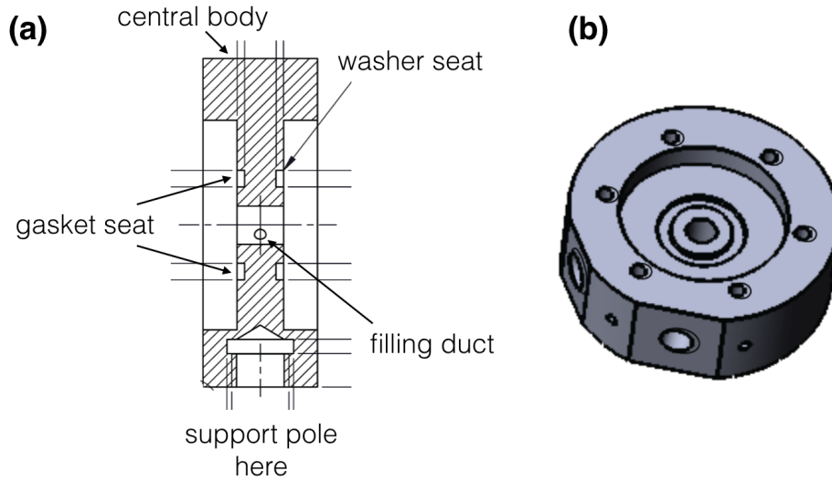
Figure 5.3 – (a) . Lateral view of the central body of the LAC. The central cylindrical duct communicates with the two seats for the lateral washers. The toroidal seats of the EPDM gaskets for the connection between washers and central body are visible. At the bottom, a thread for the supporting rod is carved. On the center of the central duct, the opening to the filling duct is visible. (b) . Three-dimensional view of the central body. The seat for the EPDM gasket, the six threads to screw the plug, the thread to screw the nut connected to the capillary, and the thread for the supporting rod are visible. Adapted from the design by the Mechanical Design Office of the LULI laboratory.
