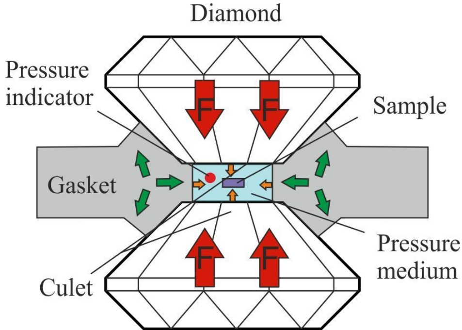
Figure 2.2 – Simplified scheme of a Diamond Anvil Cell (DAC). The coloured arrows indicate the directions in which the force of the corresponding element is exercised. Adapted from Waeselmann (2012).
