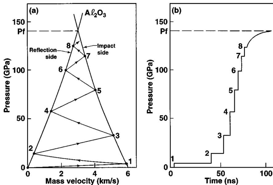
Figure 3.5 – Shock reverberation in hydrogen. The hydrogen sample is encapsulated between two sapphire ( Al_2O_3 ) windows. (a). Compression path of hydrogen in the pressure – material velocity plane. up. State 1 is reached after the first shock in hydrogen; state 2 is reached when the first shock reflects off sapphire, etc. Even-numbered states lie on the Al_2O_3 principal Hugoniot; odd-numbered states lie on the mirror reflection of such Hugoniot. (b). Pressure as a function of time at midpoint of the hydrogen sample. The time duration of each pressure step shortens as hydrogen compresses. State 1 is a shocked state; states 2 and higher are very weak shocks and comprise a quasi-isentrope. P_f is the final pressure in hydrogen, equal to the incident pressure from sapphire. From Nellis et al. (1999).
