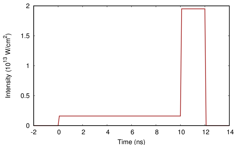
Figure 3.13 – Temporal profile of the drive laser intensity employed in the MULTI simulation. Two flat pulses have been simulated: the first is weak and long, the second is stronger and short. Each laser pulse drives a shock wave inside the sample.
