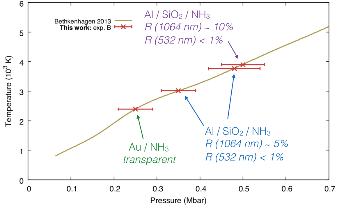
Figure 5.16 – Thermodynamic conditions reached in the low-energy shots on liquid ammonia using the temperature – pressure curve calculated by Bethkenhagen et al. (2013). For each shot, the target structure (Au / NH 3 or Al / SiO 2 / NH 3 ) and the observed optical properties (transparent or reflecting) are specified.
