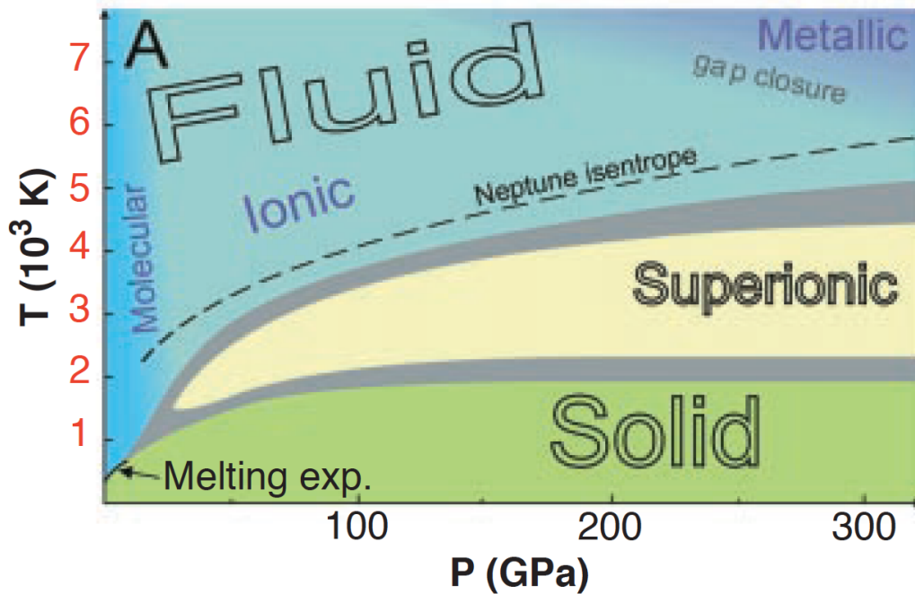
Figure 2.1 – Phase diagram of water at WDM conditions predicted in the pioneering work by Cavazzoni et al. (1999) . Despite its stoichiometric simplicity, pure water exhibits a rich phase diagram including a superionic phase between 2000 and 4000 K, a dissociated ionic phase, and an electrically-conducting, metallic-like phase at temperatures around 6000 K. The gray regions indicate the conditions in which the stable phase was not clearly determined.
