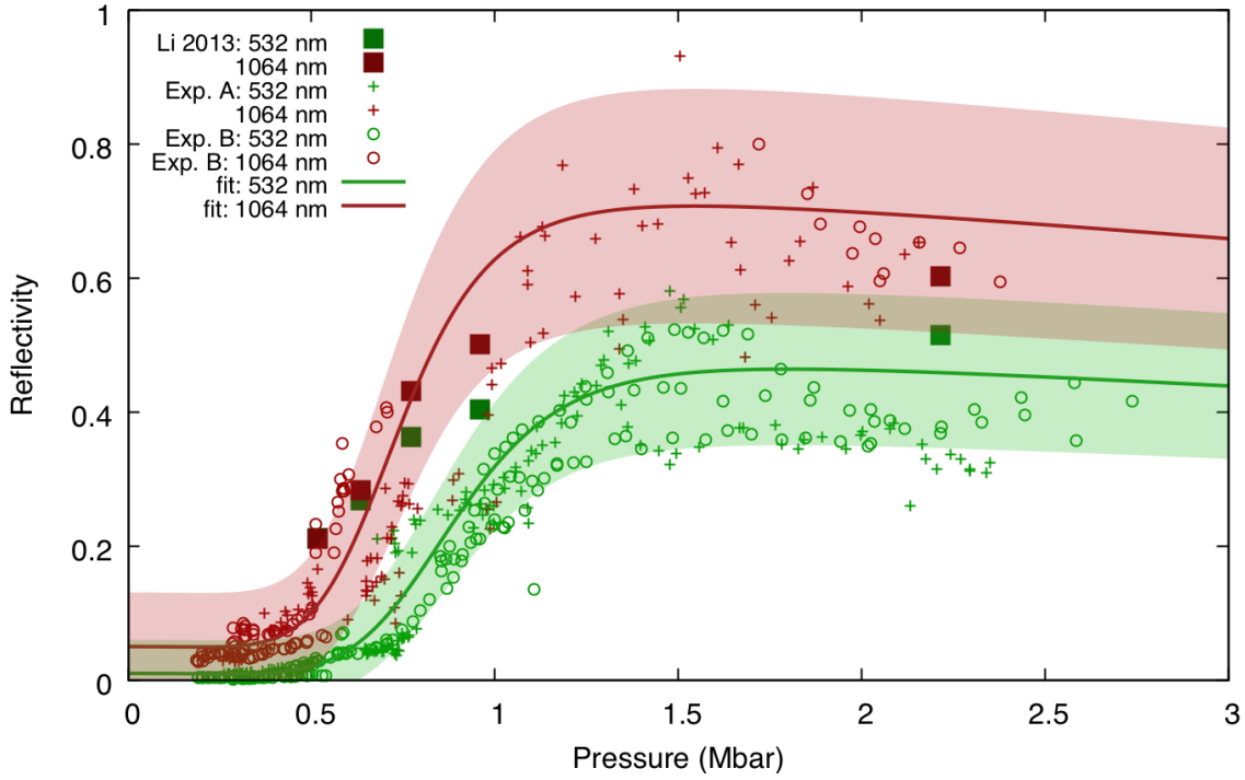
Figure 5.18 – Shock-front reflectivity at 532 nm and 1064 nm in liquid ammonia along the Hugoniot curve. Data from this work start from 0.61 g/cm 3 and ambient temperature. Calculations by Li et al. (2013) , which are also shown, start from 0.69 g/cm 3 and 230 K.
