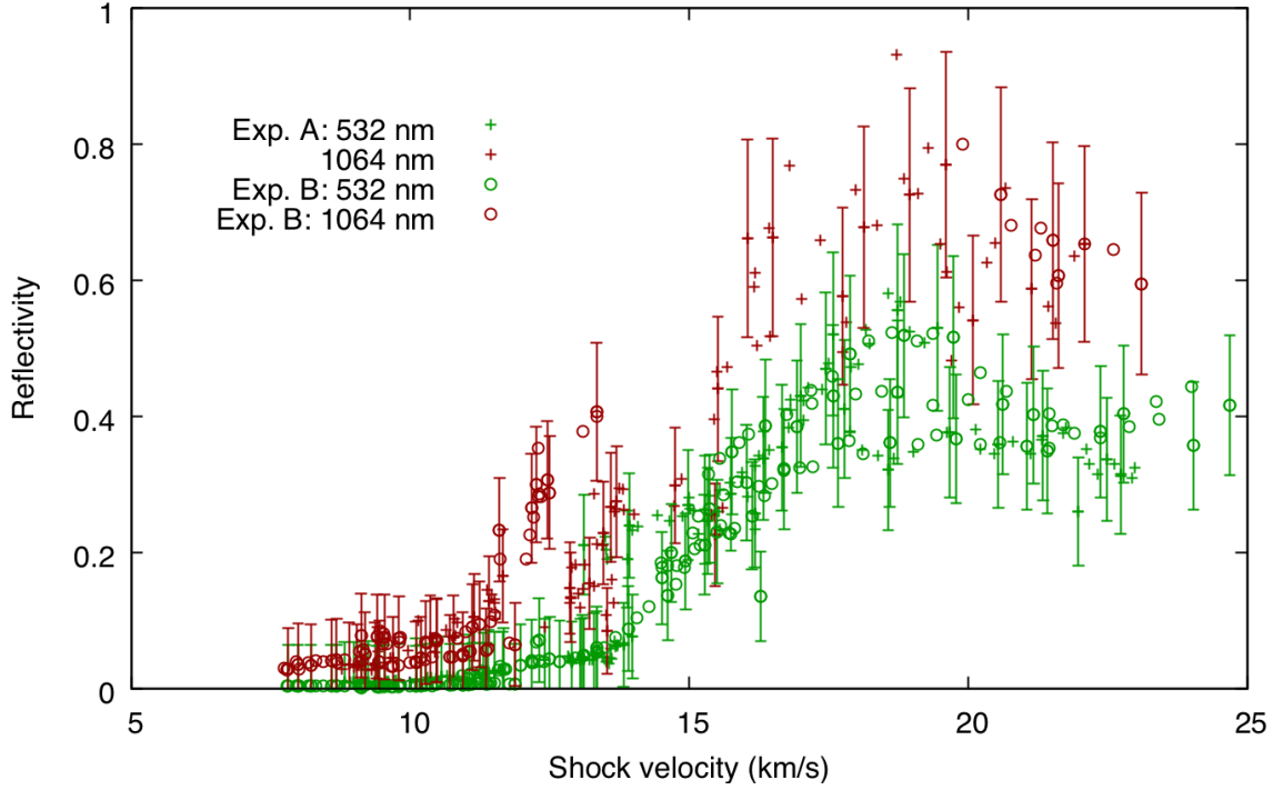
Figure 5.17 – Shock-front reflectivity at 532 nm and 1064 nm as a function of shock velocity along the ammonia Hugoniot curve starting from 0.61 g/cm 3 and ambient temperature.
