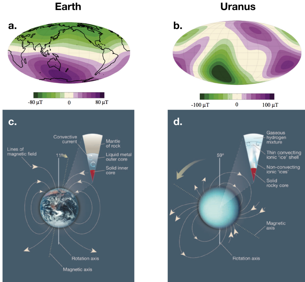
Figure 1.12 – Magnetic fields of the Earth and Uranus in comparison. (a). Radial magnetic field at the Earth surface. The colours represent field intensity; purple and green indicate the outward and inward direction, respectively. (b). Radial magnetic field at the 1-bar Uranus surface. (c). Field lines for the Earth magnetic field. The inset highlights the dynamo-active layer of the planetary interior: the liquid outer core. (d). Field lines for the Uranus magnetic field. The inset identifies a thin convecting icy shell as the dynamo-active layer in the planet's interior. (a) and (b) from Schubert and Soderlund (2011). (c) and (d) from Aurnou (2004). Magnetic field data shown in plot (a) are from Holme and Bloxham (1996). Those shown in plot (b) are elaborated by the working group V-MOD: Geomagnetic Field Modeling of the International Association of Geomagnetism & Aeronomy and are available online at www.ngdc.noaa.gov/IAGA/vmod .
