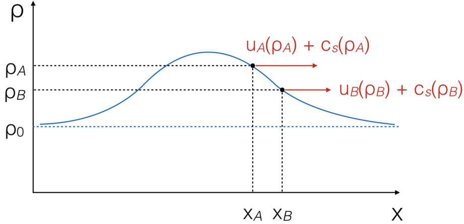
Figure 2.5 – Arbitrary finite-amplitude density perturbation to an equilibrium state \rho_0 .
