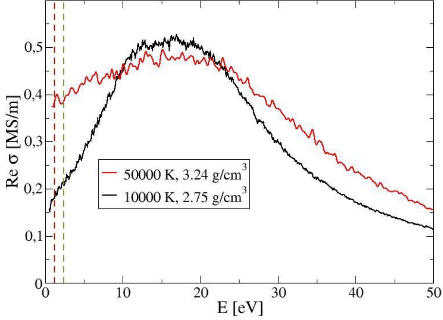
Figure 4.18 – Real part of the electrical conductivity of pure water as a function of photon energy for two principal-Hugoniot conditions: at 10 kK (black curve) and at 50 kK (red curve). At 10 kK, the behaviour is clearly not Drude-like, as the slope is initially positive and the curve reaches a maximum at around 15 eV. The ratio between the zero-energy and the maximum value is around 29%. Even at 50 kK, the initial slope is slightly positive revealing a non-Drude-like behaviour. However the ratio becomes closer to 1 (about 79%). Personal communication by Martin French ( University of Rostock ). The energies corresponding to the wavelengths of 1064 nm and 532 nm (1.17 eV and 2.33 eV, respectively) are highlighted by the red and green dashed lines, respectively.
