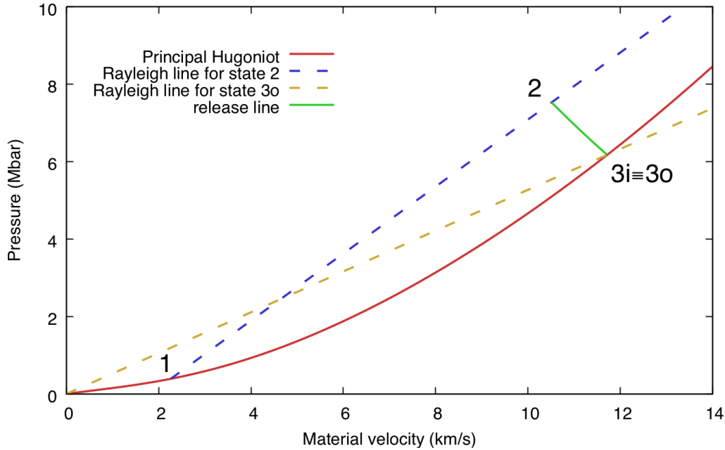
Figure 6.8 – Application of the self impedance mismatch, as detailed in Chapter 3.3.3, for the determination of state 2 for shot A-40. States 1 and 3 are identified along the principal Hugoniot of \alpha -quartz. State 3 identifies two different states, 3o and 3i, with the same material velocity and pressure. A Rayleigh line is traced from state 1, with a slope depending on the measurement of the second-shock velocity. An adiabatic compression curve is traced from state 3, using the mirror-Hugoniot approximation. State 2 is identified as the intersection of the two curves.
