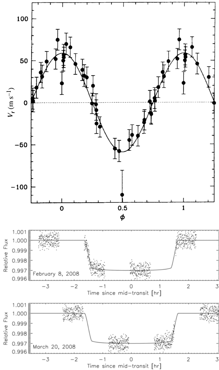
Figure 1.7 – Detection methods for exoplanets. Top. Radial velocity. Orbital motion (radial velocity vs phase) of 51 Peg. The solid line represents the computed motion. From Mayor and Queloz (1995) . Bottom. Transit photometry. Infrared photometry by the Hubble Space Telescope [ nasa.gov/hubble ] of two transits of the exoplanet HD 149026b. Interruptions are due to Earth occultations. The solid curve is the best-fitting model. From Carter et al. (2009) .
