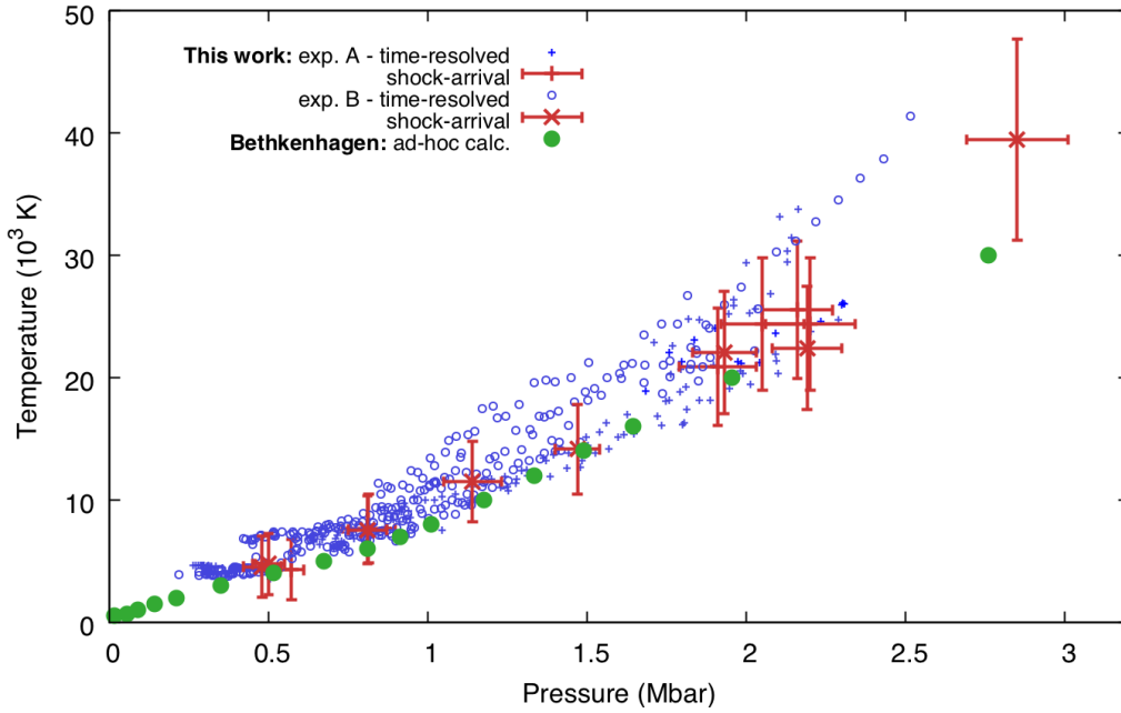
Figure 5.14 – Comparison between experimental data of this work and calculations by Mandy Bethkenhagen along the Hugoniot of ammonia starting from 0.61 g/cm 3 and 300 K in the temperature – pressure plane.
