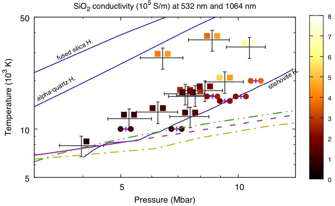
Figure 6.16 – Optical conductivities of warm dense silica. Grey crosses are the conditions experimentally explored via double-shocks; violet crosses are the conditions simulated by F. Soubiran. Coloured squares (experimental data) and circles (calculations) on the left and right side of the crosses express the conductivity at 1064 nm and 532 nm, respectively, according to the colour scale. The melting curves of silica are the same as in Figure 6.9.
