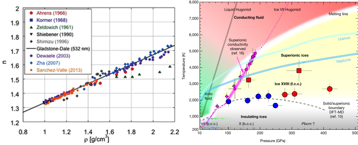
Figure 4.1 – Left. Water refractive index along the principal Hugoniot curve as a function of density. From Batani et al. (2015) . Right. Water phase diagram in the WDM regime. From Milot et al. (2019) .
