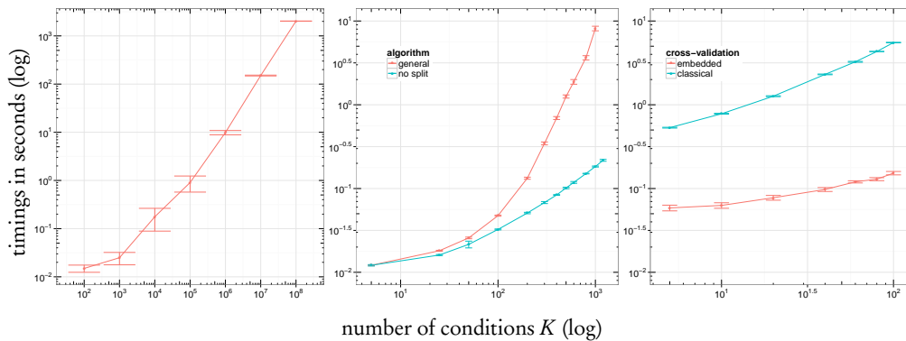
Figure 3.21 – timing experiments: a) time in seconds as a function of the number of conditions K ; b) timing comparison for general/without-split algorithm; and c) timing comparison for naive/embedded cross-validation.
