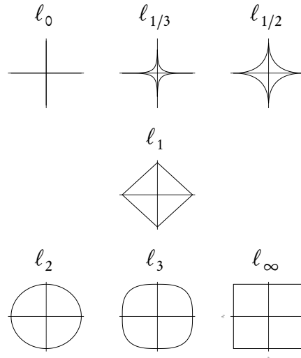
Figure 3.2 – Contour of the feasible sets defined by \|\beta\|_\gamma \leq 1 for various values of \gamma when \beta \in \mathbb{R}^2 .
