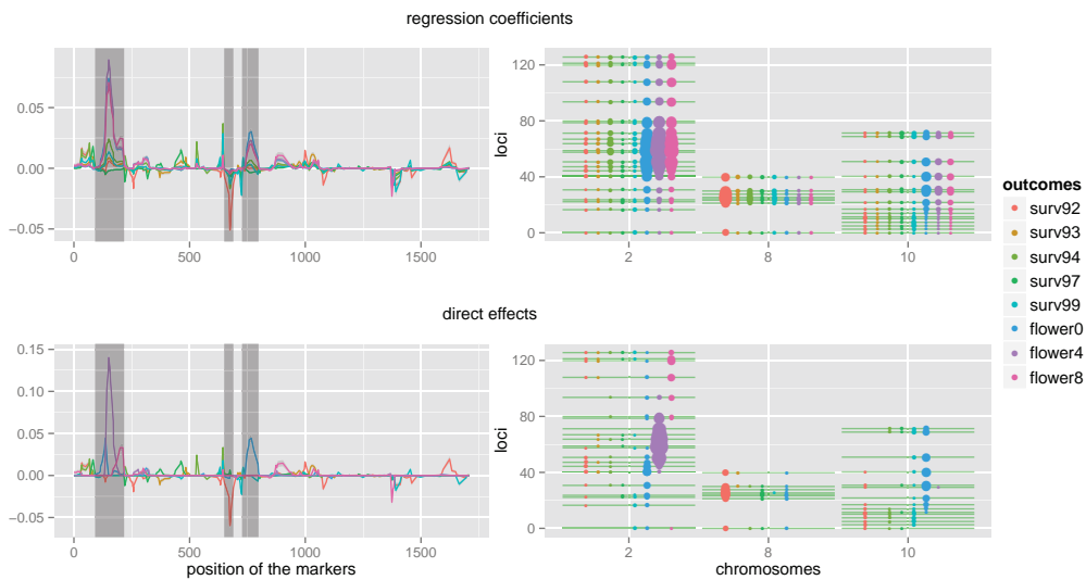
Figure 3.14 – Brassica Study: direct and indirect genetic effects of the markers on the traits estimated by SPRING (better seen in color).
