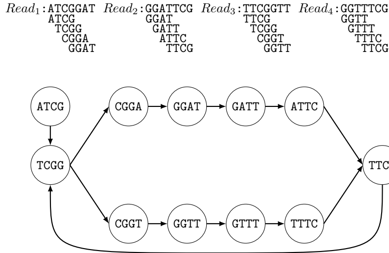
Figure 3.11: We have a dataset of 4 reads with length equal to 7, we choose a value of k equal to 4, k -mers are present under each read. A DBG built from this k -mer set is present under reads, each node is a k -mer and if a word shares k - 1 symbol at its end with k - 1 symbols at the beginning of another node, we build a directed edge. This DBG contains a cycle. This cycle probably matches a repetition in the original sequence.
