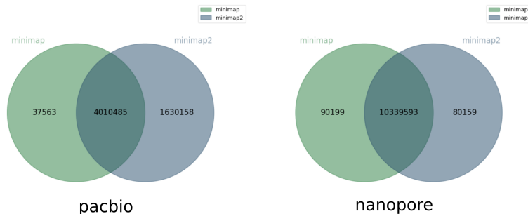
Figure 2.8: Jaccard similarity 0.71, 0.98
