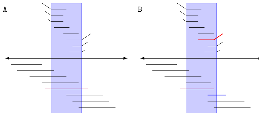
Figure 3.7: Black arrow line was the path chosen by Canu , the other line was a read mapped against this path, the blue box indicates a repeat region. In case A the purple read spans all the repetition and indicates that the path chosen by Canu was the good one. In case B no read spans the repetition and the purple read have non-congruent overlaps between the red and blue reads, so Canu needs to break the path in order not to create a misassembly
