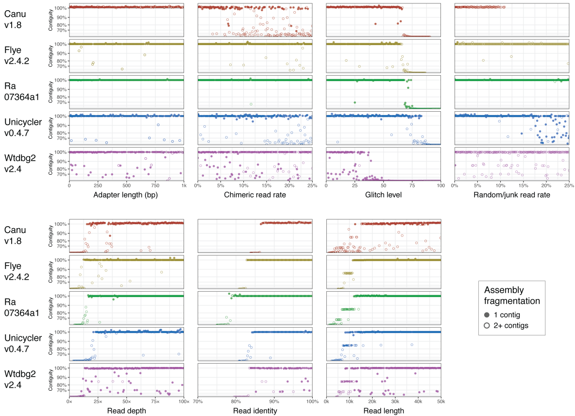
Figure 4.12: Effect of different reads property on assembly contiguity (number of contigs expect and map correctly on reference genome), of five assembly tools. Unicycler is an hybrid assembler (use second and thrid generation read). Canu is a long-read assembly pipeline they perform a self correction before construct assembly with a special OLC graph (more detail in Section 3.5). Ra perform a basic string graph assembly on raw reads with a correction of contigs after assembly (more detail in Section 3.6). wtdbg2 and Flye use a DBG like approach to perform assembly on raw reads (more detail in Section 3.7). This figure is a reproduction of figure from [109].
