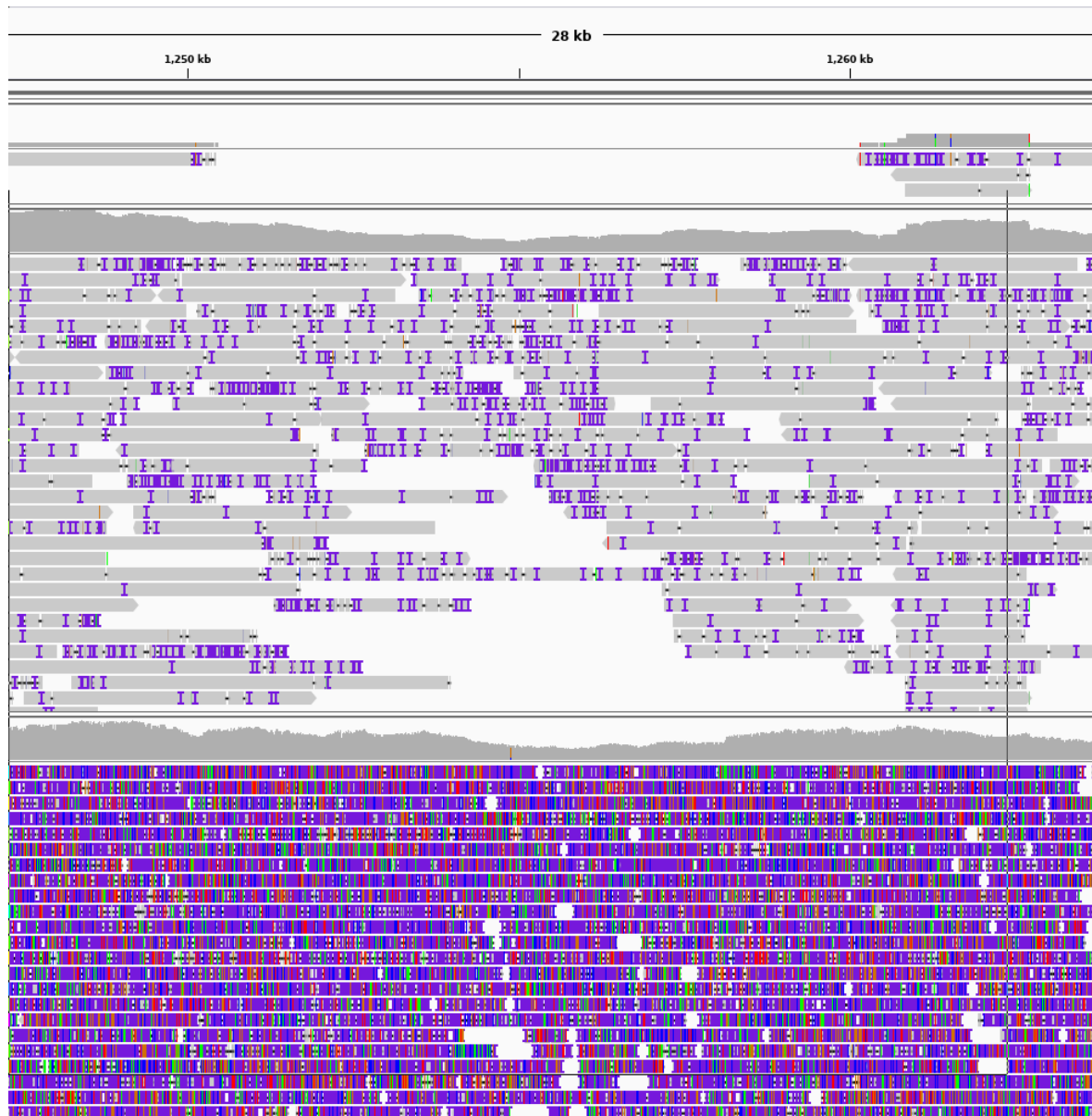
Figure A.5: IGV view of NCTC5050 mapping of Canu contig against NCTC contig, in junction between tig10 (first track at left) and tig23 (first track at right), tig41 are mapped on begin of tig23 in forward and reverse. The second track represent the mapping of Canu corrected read, the third track represent the raw reads. Above each this track we can observe the coverage curve and drop of this curve between the tig10 and tig23, for corrected read is around 50x coverage before junction, equal to 15x at minimal, and less than 40x after junction, this value are 90x, 25x and 40x for raw read. In addition we can observe more error in corrected read on this drop of coverage.
