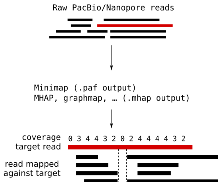
Figure A.6: YACRD (manuscript in preparation) detects chimeric regions present in the read dataset. To detect such regions, YACRD takes as input the output of an overlapper (both PAF and MHAP format are accepted). For each read in the dataset, YACRD computes positional coverage values based on the overlaps with that read. If there is a drop of coverage, the corresponding read is marked as 'chimeric'.
