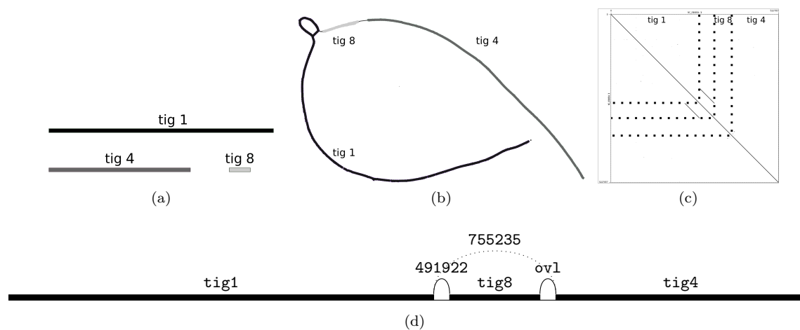
Figure 4.15: Graph analysis of a synthetic dataset ( T. roseus ). (a) Contig graph produced by Canu (visualized using Bandage ): 3 contigs, no edge. (b) SG built from Minimap2 overlaps, on which connected components of the Canu BOG are colored. (c) Dot-plot of the T. roseus genome (NC_018014.1) aligned against itself, showing a long tandem repeat. (d) The AAG with Canu contigs ordered according to their position on the T. roseus reference. If two contigs overlap, no length is given and instead the link is labeled 'ovl'.
