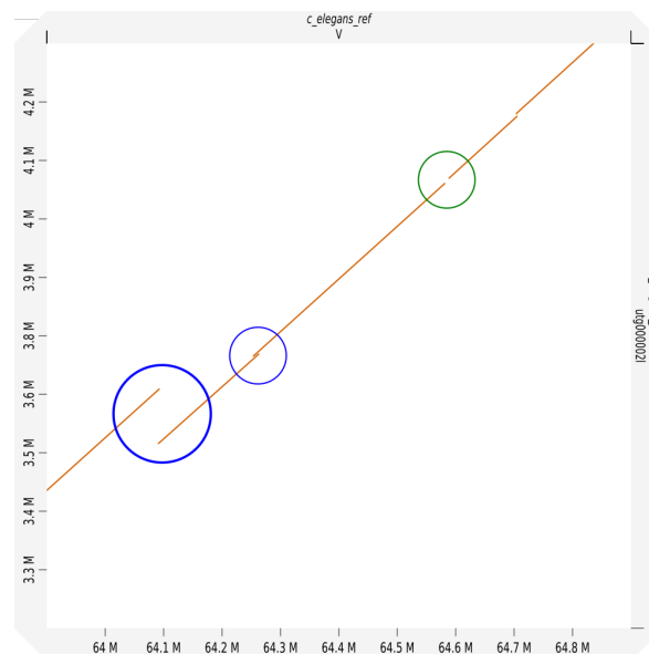
Figure 4.2: Third relocation observed in dotplot a long reads assembly against reference of C. elegans
