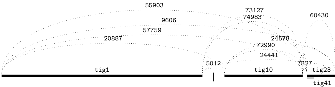
Figure A.4: NCTC5050 contigs mapped against NCTC reference for ordering. Paths are shown along with their number of bases as labels. The NCTC assembly consists of two contigs, hence the relative order of tig1 and tig10/tig23 cannot be inferred (vertical line in the figure). We observed that a portion of tig1 is inverted with respect to the NCTC assembly, with no impact on the path analysis as this putative misassembly does not involve an extremity of the contig.
