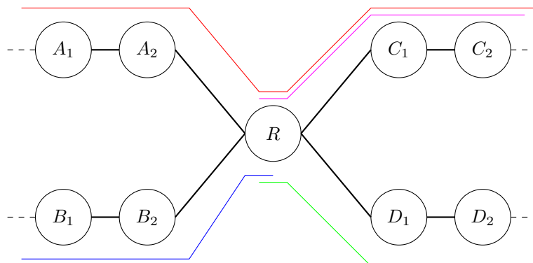
Figure 3.4: We have a part of assembly graph node R represent a repetition node A , B , C , D represent basic sequence. Red, purple, green and blue line represent reads. Red read was larger than repetition and span over it and indicate A_1 \rightarrow A_2 \rightarrow R \rightarrow C_1 \rightarrow C_2 was a good path, with out this read we can solve this repetition.
