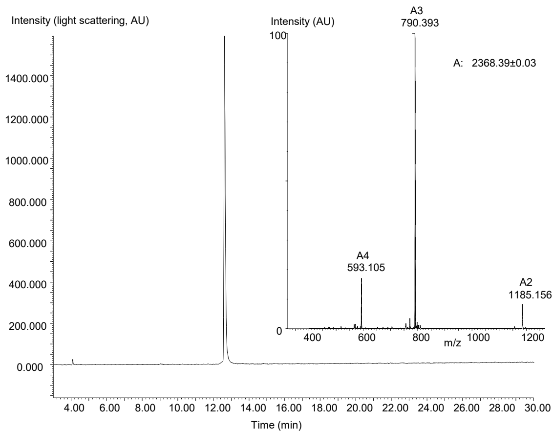
Figure S26. LC-MS analysis of peptide 21 . LC trace, eluent A 0.10 % TFA in water, eluent B 0.10% TFA in CH 3 CN/water: 4/1 by vol. C18 Xbridge BEH 300 Å 5 μm (4.6 x 250 mm) column, gradient 0-100% B in 30 min (1 mL/min, detection 215 nm). MS trace: M calculated (mean) 2368.84, found 2368.39±0.03.
