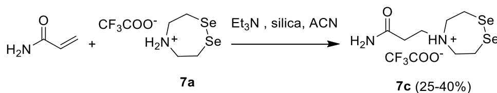
Scheme S3. Synthesis of N -(2-carboxamidoethyl) bis(2-selenylethyl)amine 7c .
