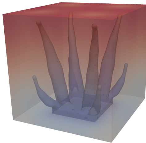
Figure 6.13: Optimized 3-d design for heat conduction obtained with the surface expression of the shape derivative (test case of section 6.2.2).
