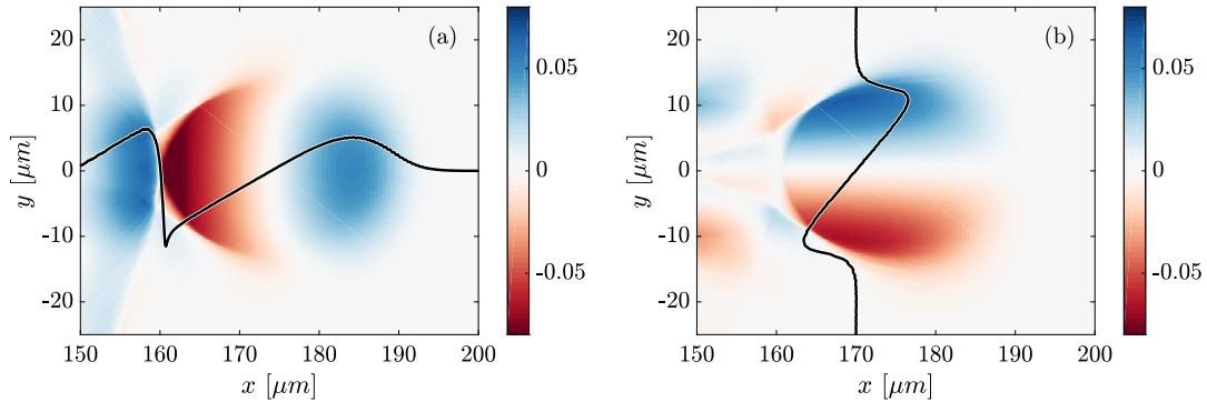
Figure 2.19: Same simulation and instant than Fig. 2.18. (a) Longitudinal field E_x [ m_e c \omega_0 / e ] (colormap) and on-axis profile (black line) of the electronic bubble. (b) Transverse force E_y - cB_z [ m_e c \omega_0 / e ] (colormap) and transverse profile at x = 170 \mu\text{m} (black line).
