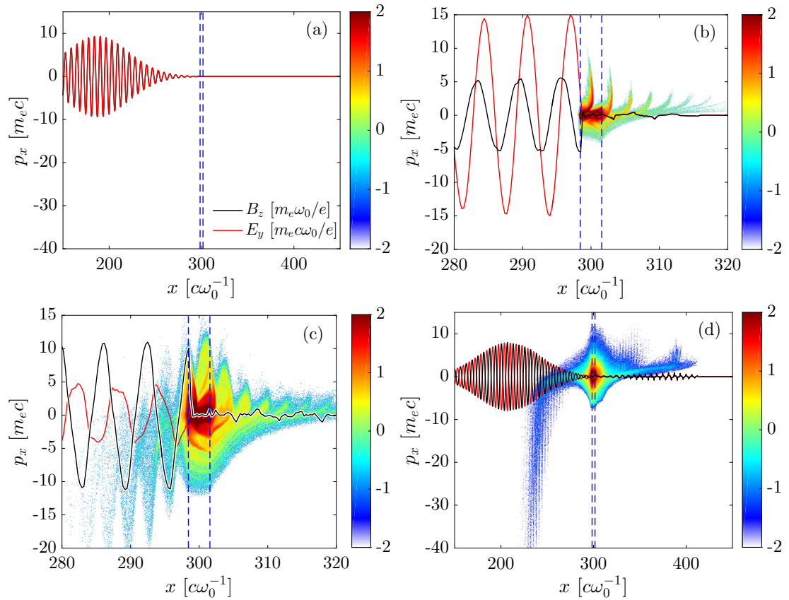
Figure 5.14: Overlap of the longitudinal electron phase space map ( x, p_x ) and of the on-axis ( E_y, B_z ) laser fields at (a) t = 300 \omega_0^{-1} , (b) t = 400 \omega_0^{-1} , (c) t = 440 \omega_0^{-1} and (d) t = 500 \omega_0^{-1} for the 500 nm thick plastic target. The vertical blue dashed lines represent the initial target limits. Note the change of scale in (a,d) compared to (b,c).
