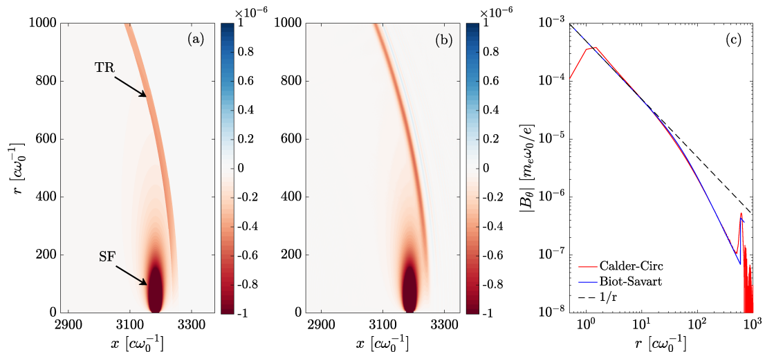
Figure 3.14: Comparison between results of (a) the Biot-Savart model and (b) the PIC code CALDER-CIRC simulating a rectangular electron bunch with length L_b = 3 \mu\text{m} and \gamma = 5 emerging from a perfect conductor into vacuum. (c) Radial cut profile at x = 3250 c\omega_0^{-1} from CALDER-CIRC results (red line) and Biot-Savart model (blue line), compared to 1/r decay (black dashed line).
