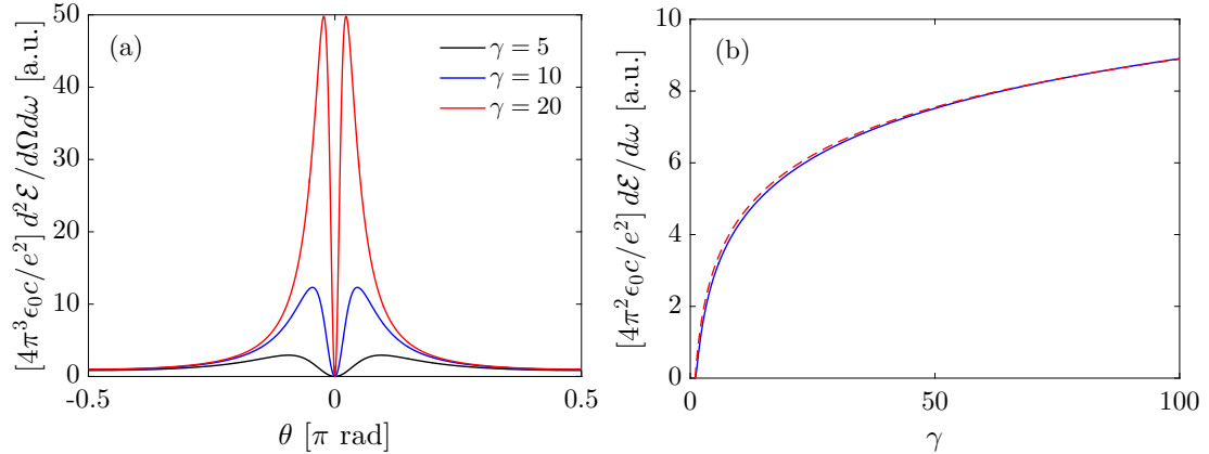
Figure 2.24: (a) Angular emission of TR according to Eq. (2.262) emitted by an electron exiting a perfect conductor for different \gamma factor. (b) Integration over \theta angle of the radiated energy (blue line) with a \ln(\gamma) law (red dashed line).
