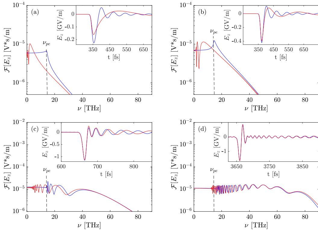
Figure 2.10: THz spectra and fields (see insets) at different propagation distances computed from the MAXFLU1D code (blue curves) and the UPPE1D code (red curves) for a two-color 50-fs Gaussian pulse with 150 \text{ TW}/\text{cm}^2 intensity: (a) x = 3 \mu\text{m} (corresponding to almost one plasma skin depth \delta_{pe} ), (b) x = 10 \mu\text{m} , (c) x = 100 \mu\text{m} , and (d) x = 1 \text{ mm} . Vertical dashed lines indicate \nu = \nu_{pe} .
