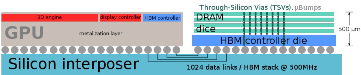
Figure 1.2: Sub-part of a cut through a graphics card that uses High Bandwidth Memory. Grey dots represent: PCI express / Electrical current / Display connectors. Source: https://en.wikipedia.org/wiki/High_Bandwidth_Memory
