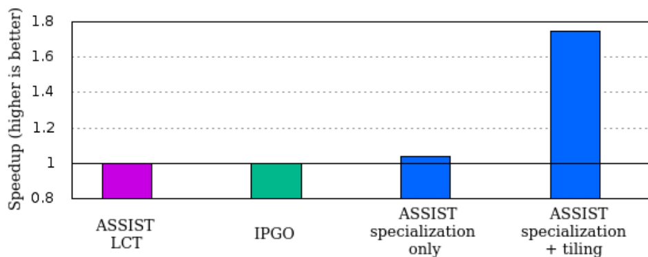
Figure 4.11: ABINIT - Ti-256 - Speedups of IPGO, ASSIST LCT, specialized with ASSIST, specialized and tiled with ASSIST compared to the original version
